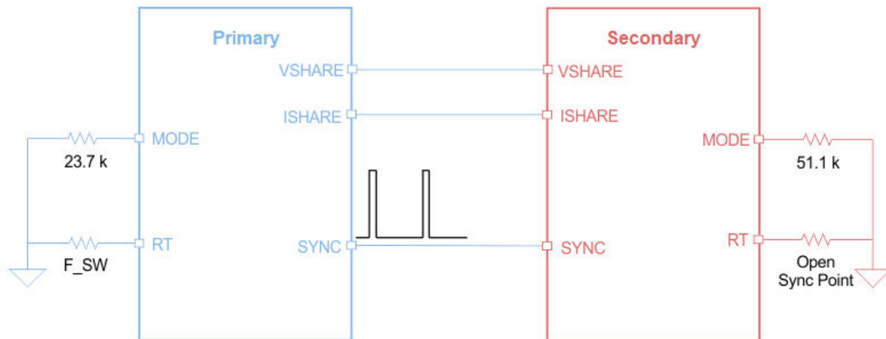
FIG 7-4. 2-Phase Stackable, 180° Phase Shift: Primary Sync-Out Clock to Secondary
