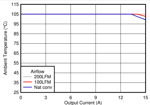
Figure 6-10. Safe Operating Area
