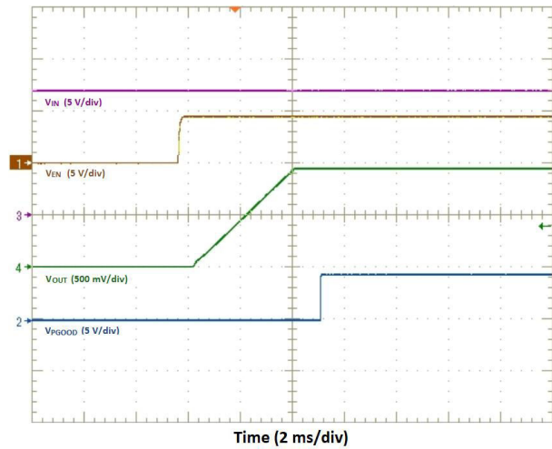
8-3. Start-Up Waveforms
