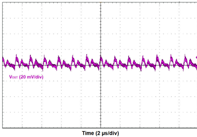
8-2. Output Ripple Waveform
