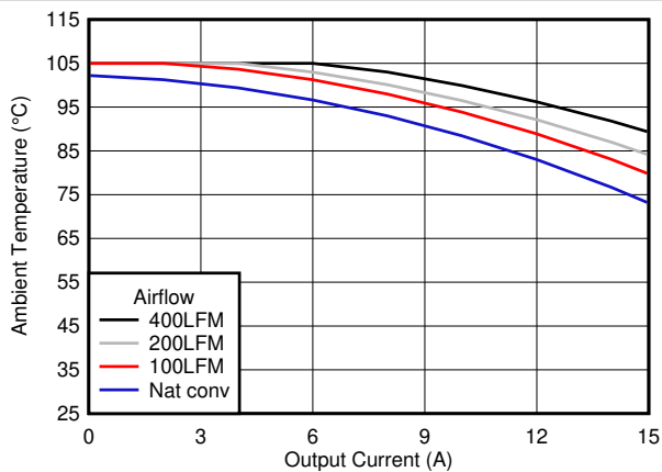
Figure 6-4. Safe Operating Area
