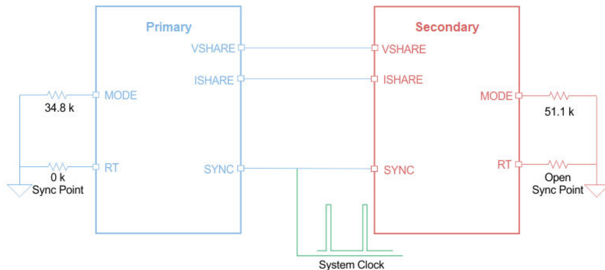
FIG 7-5. 2-Phase Stackable, 180° Phase Shift: Primary and Secondary Sync to External System Clock
