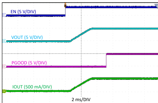
9-4. Enable Start-Up V_{IN} = 24\text{ V} , V_{OUT} = 5\text{ V} , I_{OUT} = 0.5\text{ A}
