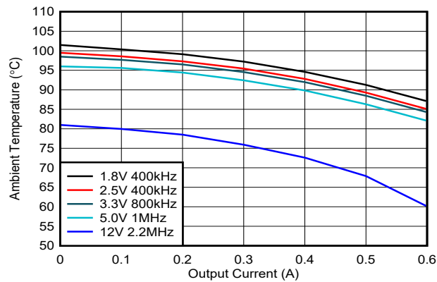
8-14. Safe Operating Area (Standard EVM Layout and Board Size)
