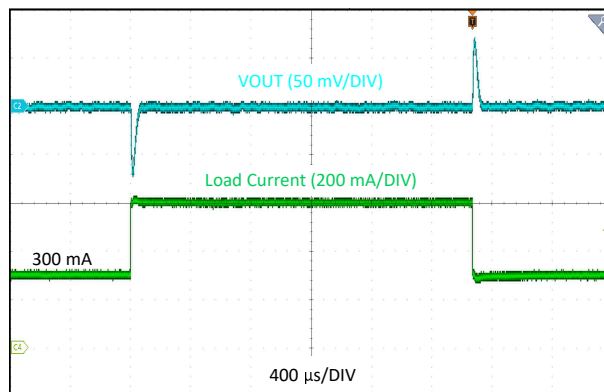
10-6. Load Transient, 0.3 A to 0.6 A, 1 A/μs
