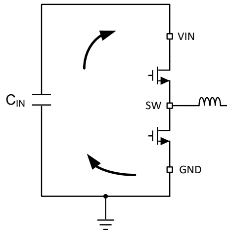
FIG 10-14. Current Loops with Fast Edges
