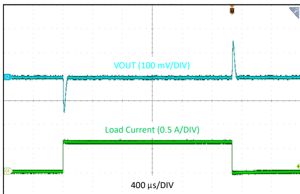
10-5. Load Transient, 0 A to 0.6 A, 1 A/μs
