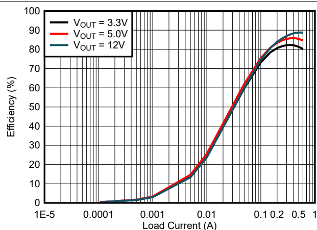
8-10. Efficiency in FPWM Mode
