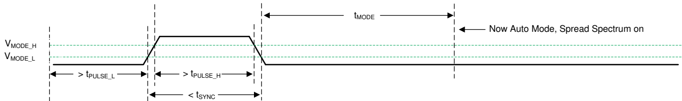
図 9-7. Transition from SYNC Mode to Auto Mode
