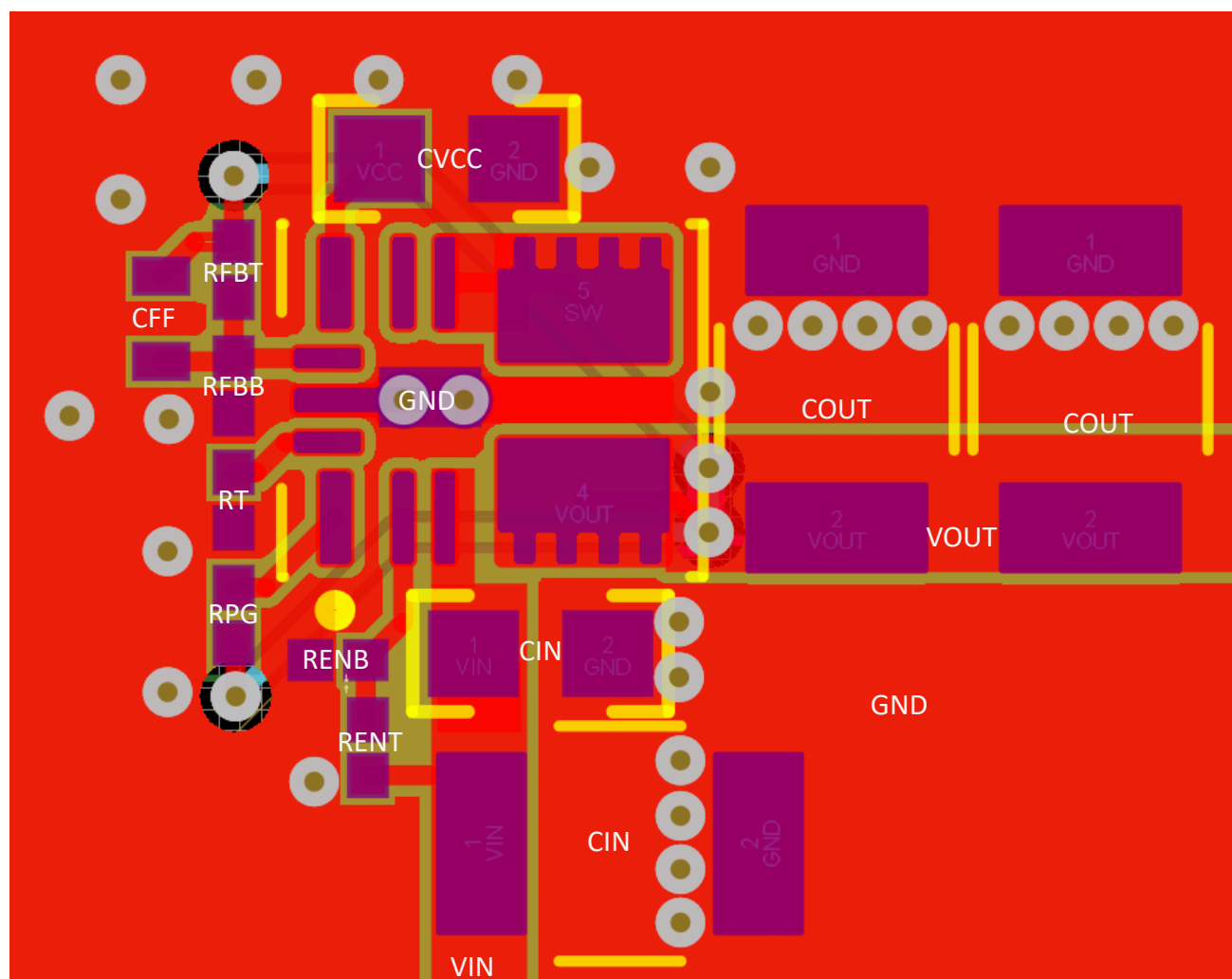
10-15. Example Layout
