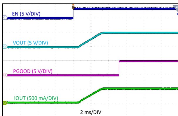
10-3. Start-Up Waveforms
