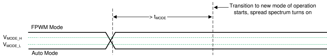
図 9-6. Transition from Auto Mode and FPWM Mode
