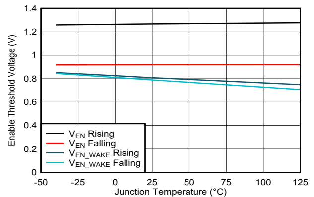
Figure 8-4. Enable Thresholds
