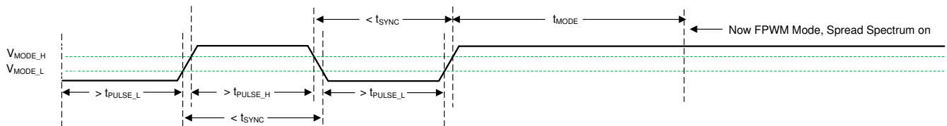
図 9-8. Transition from SYNC Mode to FPWM Mode
