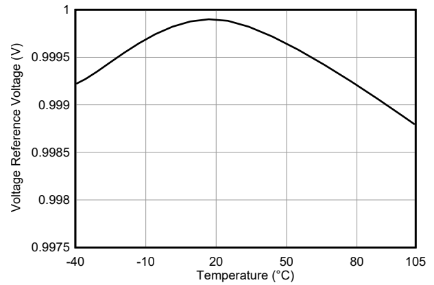
6-2. Feedback Voltage ( V_{FB} ) Accuracy Versus Temperature
