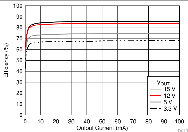
Figure 6-16. Efficiency
