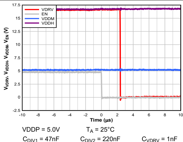
Figure 6-4. t_{HL\_VDRV}
