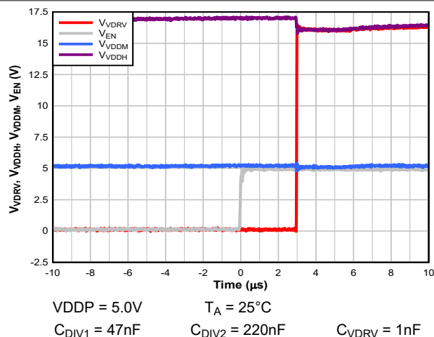
Figure 6-3. t_{LH\_VDRV}
