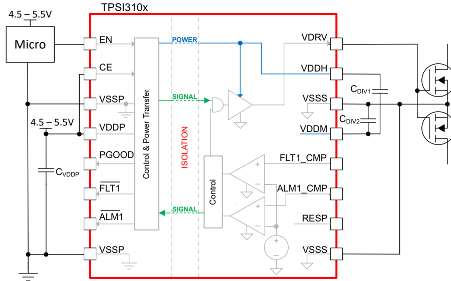
8-10. Simplified Schematic
