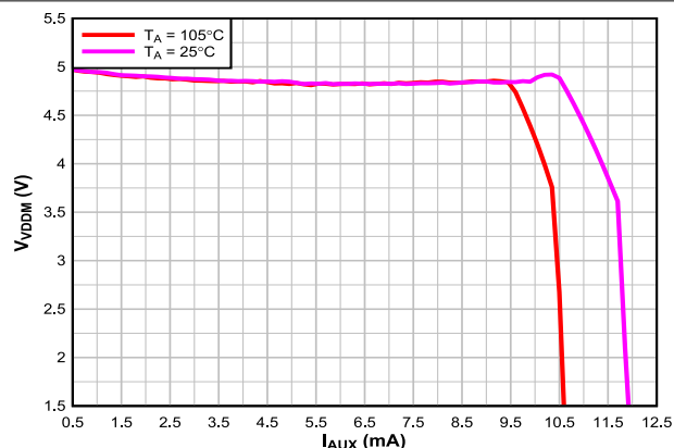
図 6-10. V_{\text{VDDM}} versus I_{\text{AUX}}
