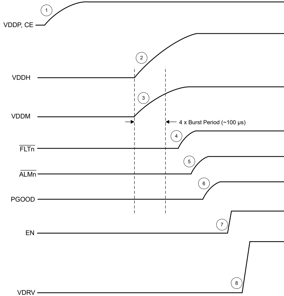
図 8-11. TPSI310x Typical Start-up (CE = VDDP, \overline{\text{FLTn\_CMP}} = 0 , \overline{\text{ALMn\_CMP}} = 0 )
