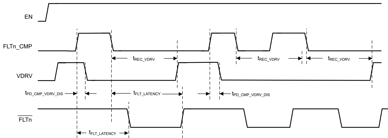
FIG 7-3. VDRV Auto-Recovery Timing (CE = 1 or CE = VDDP)
