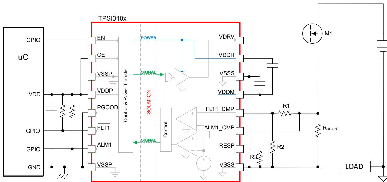
9-6. Typical Overcurrent Protection Application
