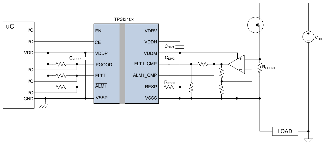
図 9-2. TPSI310x overcurrent protection with current sense amplifier, fault and alarm indicators
