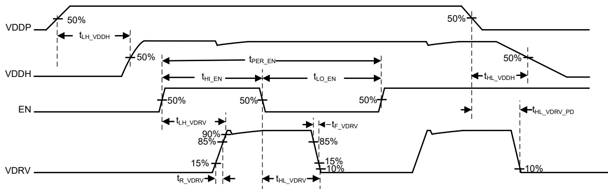
FIG 7-1. VDRV Timing, (CE = 1 or CE = VDDP, FLTn_CMP = ALMn_CMP = 0)
