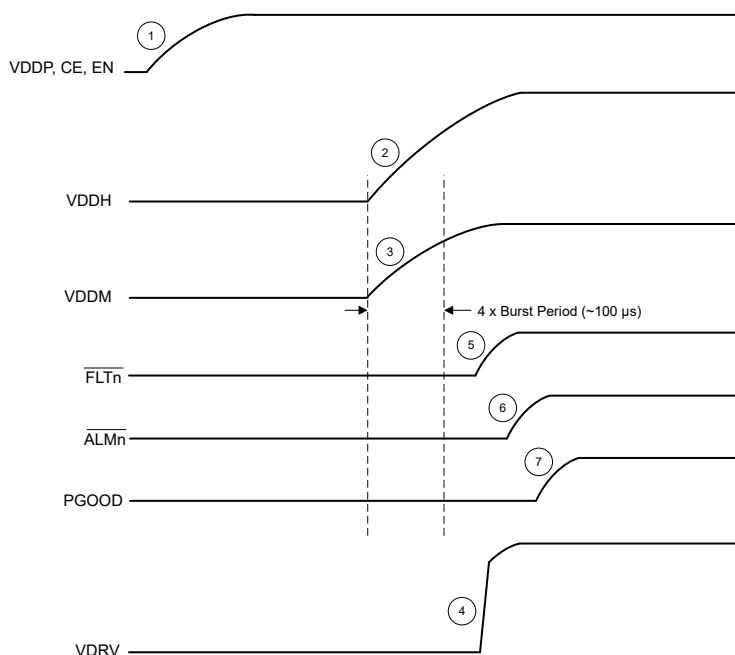
図 8-12. TPSI310x Typical Start-up (CE = EN = VDDP, FLTn_CMP = 0, ALMn_CMP = 0)
