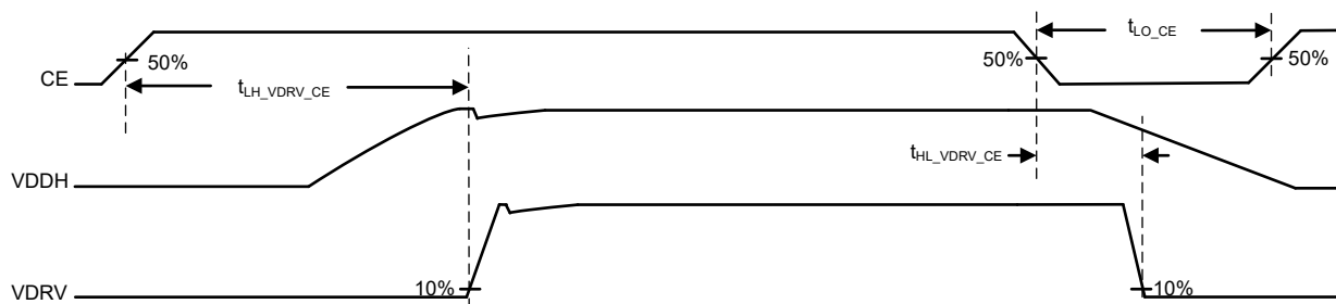
FIG 7-2. VDRV Timing, (VDDP present, FLTn_CMP = ALMn_CMP = 0)
