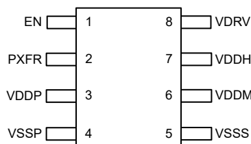
図 5-1. TPSI3052, TPSI3052S 8-Pin SOIC Top View
