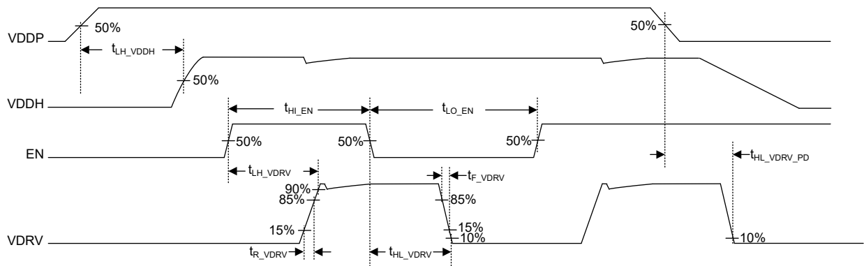
図 7-2. Three-Wire Mode Timing, Standard Enable (TPSI3052 Only)
