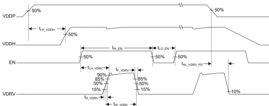
図 7-3. Three-Wire Mode Timing, One-Shot Enable (TPSI3052S Only)
