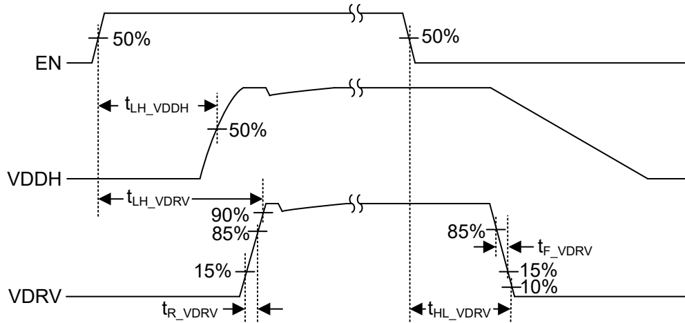
図 7-1. Two-Wire Mode Timing, Standard Enable (TPSI3052 Only)
