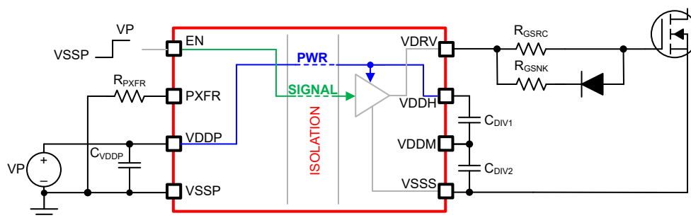
9-1. TPSI3052 Three-Wire Mode Driving MOSFETs
