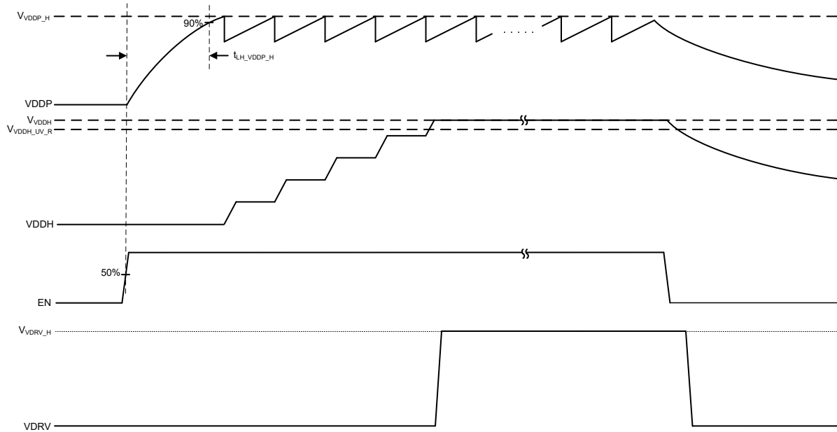
図 8-5. Two-Wire Mode with Standard Enable (TPSI3052 Only)
