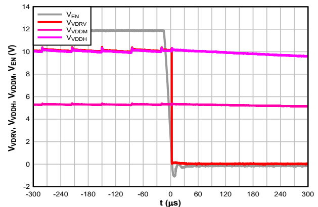
Two-wire mode EN = 12 V R PXFR = 7.32 kΩ C DIV1 = 30 nF C VDRV = 100 pF T A = 25°C C DIV2 = 100 nF
