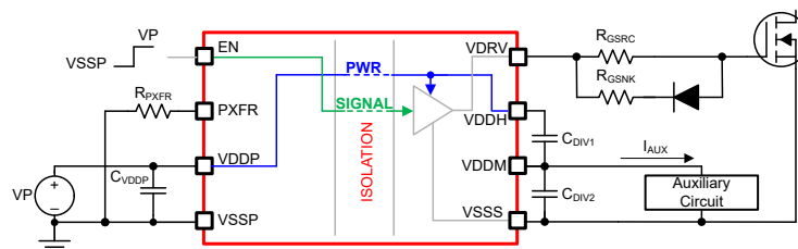
☒ 9-3. Supplying Auxiliary Power From VDDM
