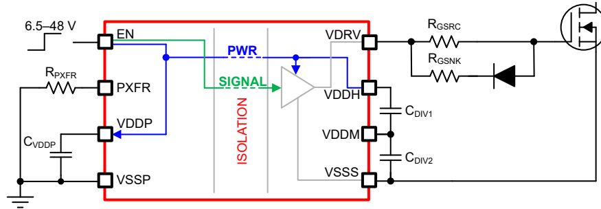
図 9-2. TPSI3050-Q1 Two-Wire Mode Driving MOSFETs
