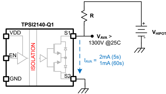
图 9-10. Dielectric Withstand Test (HiPot) - Simplified Schematic
