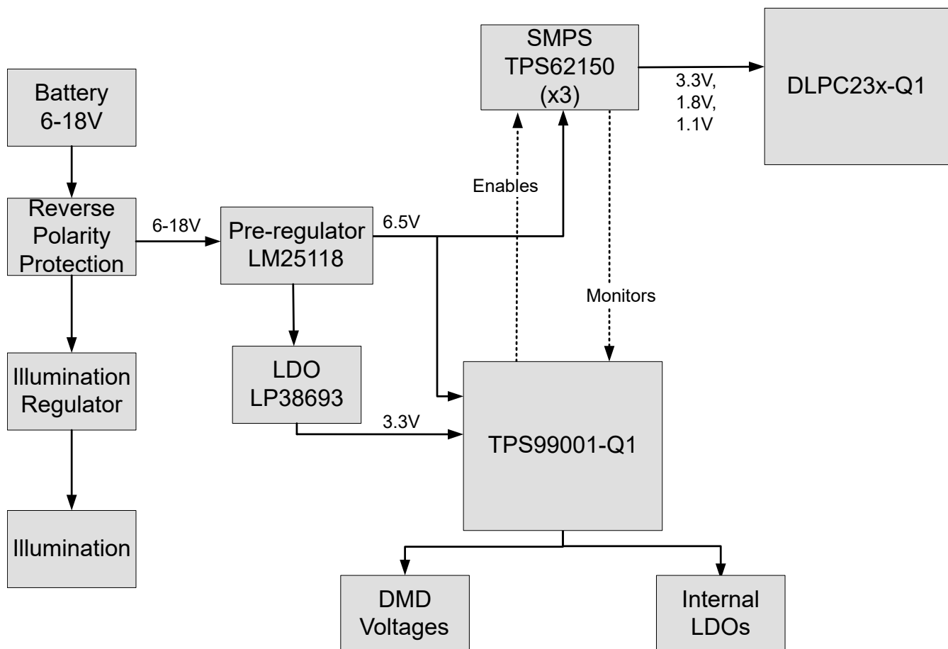
図 8-1. Headlight Power Supply Architecture
