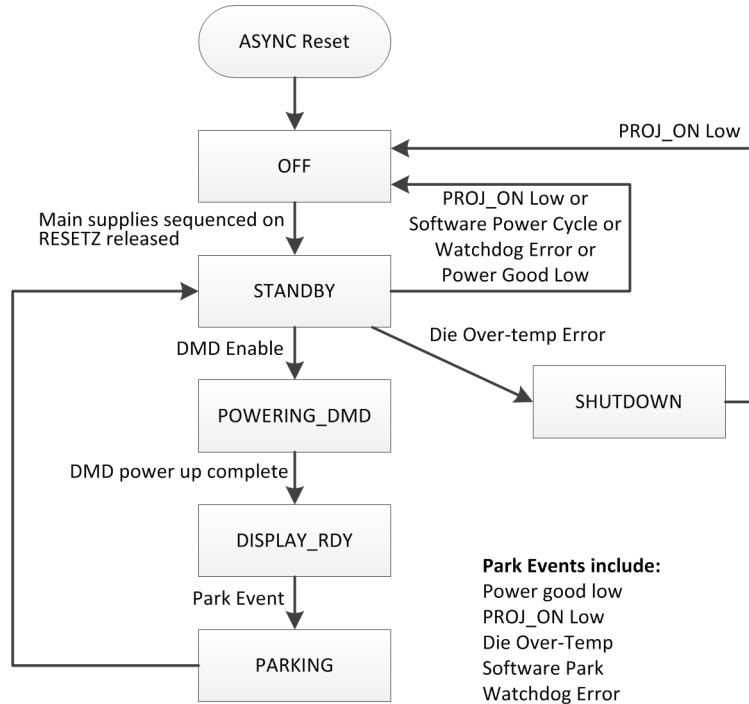
Figure 6-8. Top Level System States
