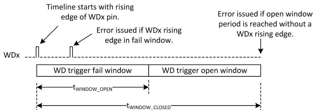
❏ 6-6. Windowed Watchdog Function
