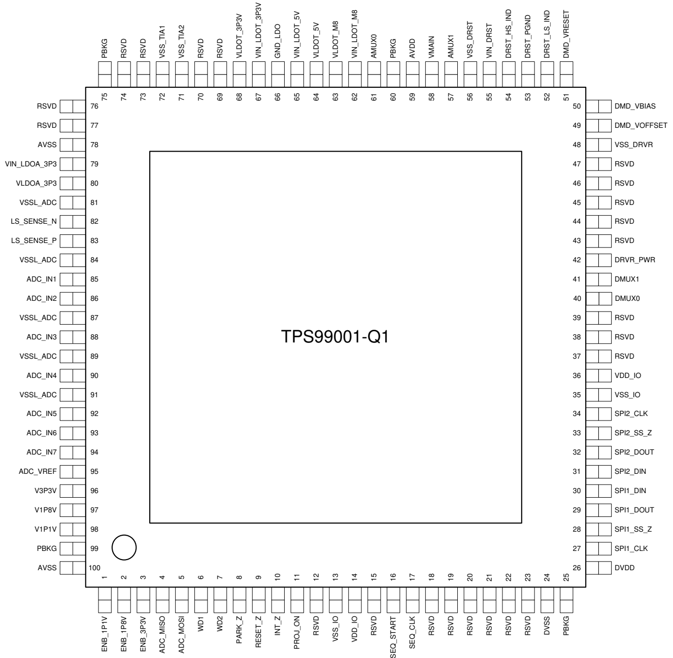
図 4-1. PZP Package 100-Pin HTQFP Top View
