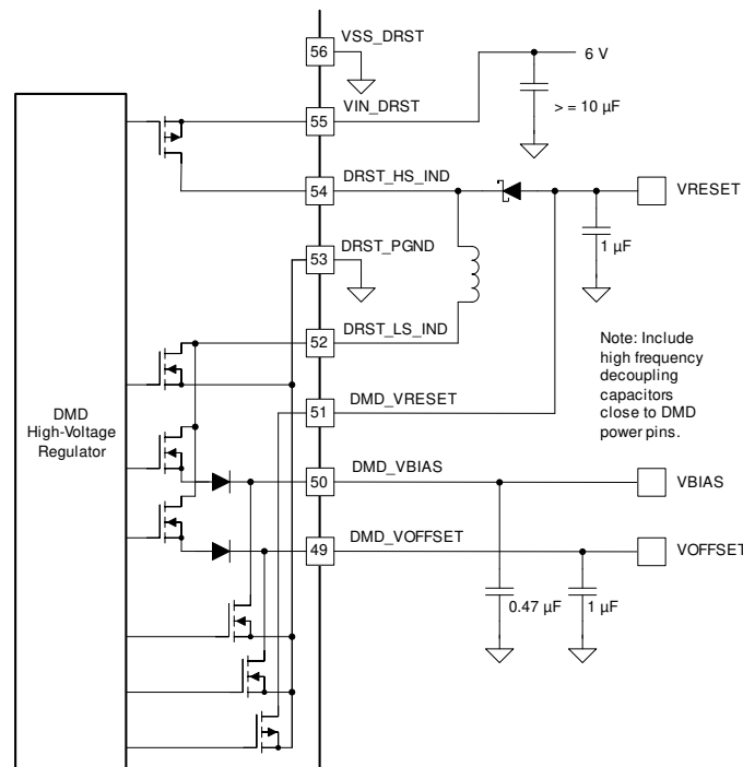
6-5. DMD Voltage Regulator Circuit
