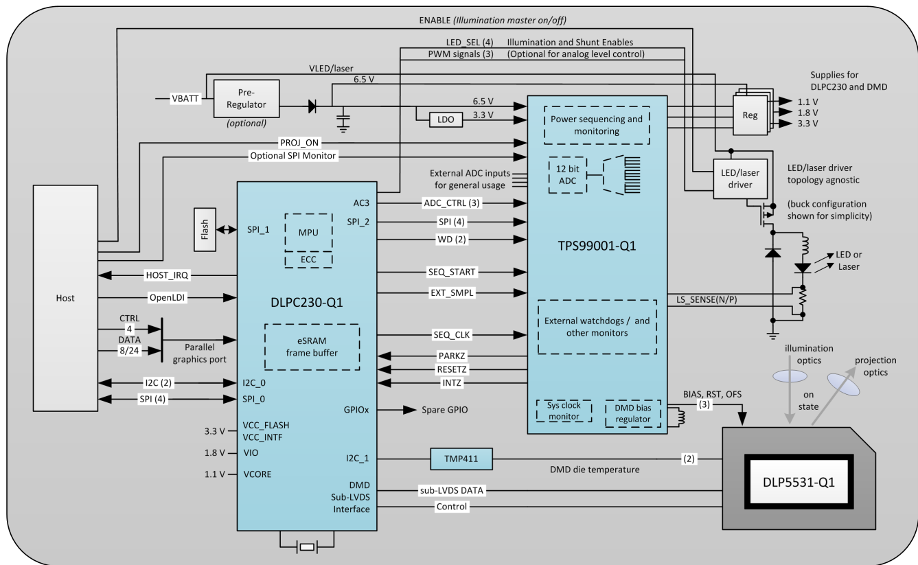
図 7-1. Headlight System Block Diagram
