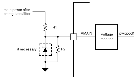
図 6-3. VMAIN Brown Out Monitor
