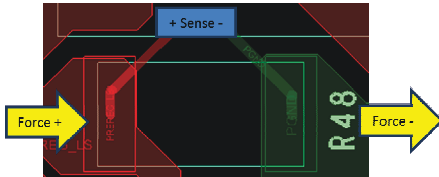
図 9-1. Kelvin Sensing Layout
