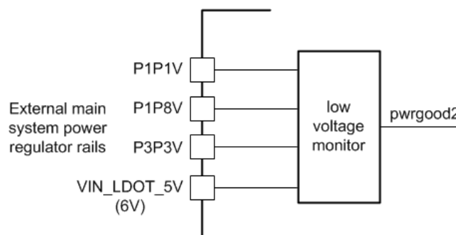
図 6-4. Real-Time Power Rail Monitors
