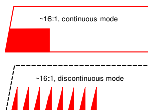
FIG 6-1. Comparison of Continuous and Discontinuous Mode Operation
