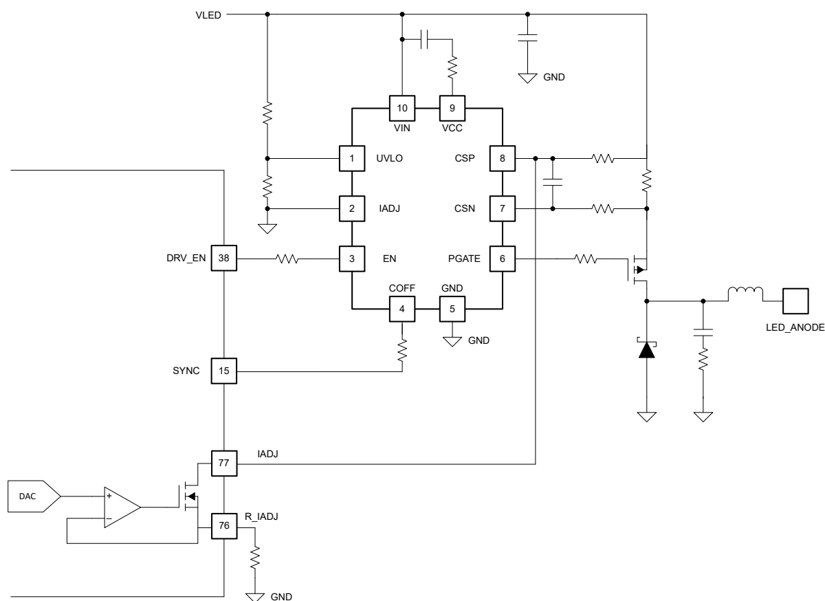
6-14. IADJ Peak Current Limit Schematic
