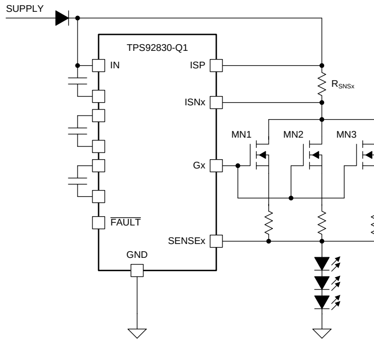
FIG 36. Parallel MOSFET Driving
