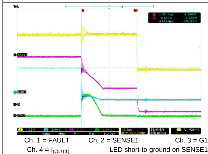
FIG 18. LED Hard Short Protection and One-Fails-All-Fail
