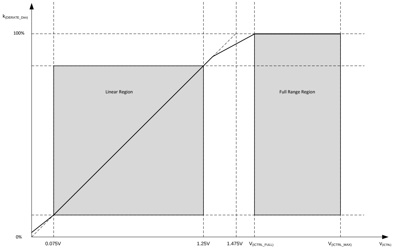
FIG 26. Analog Dimming Ratio
