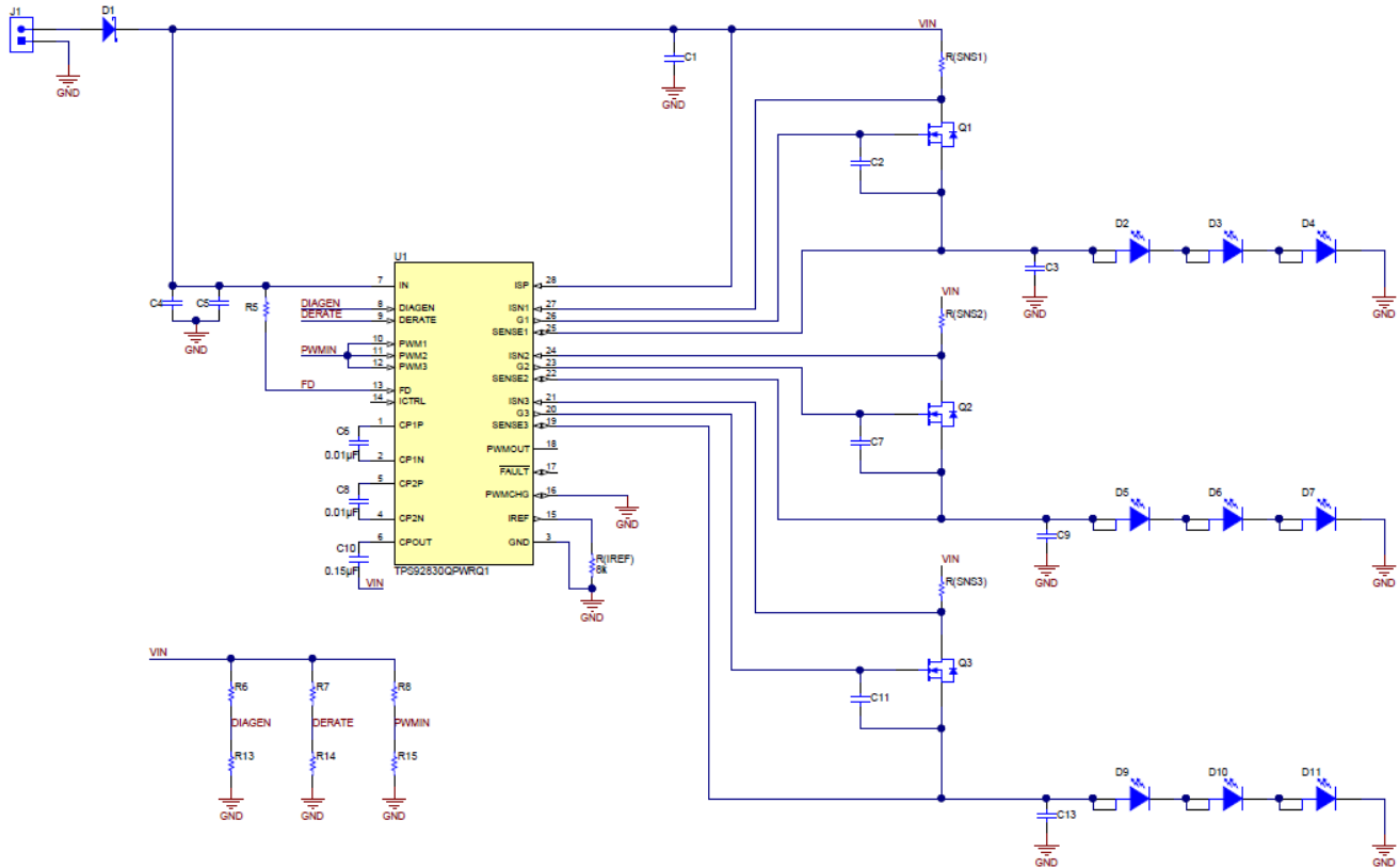
图 31. TPS92830-Q1 Typical Application Circuit For Automotive Exterior Lighting
