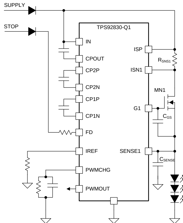
FIG 21. MOSFET Gate Capacitance Compensation
