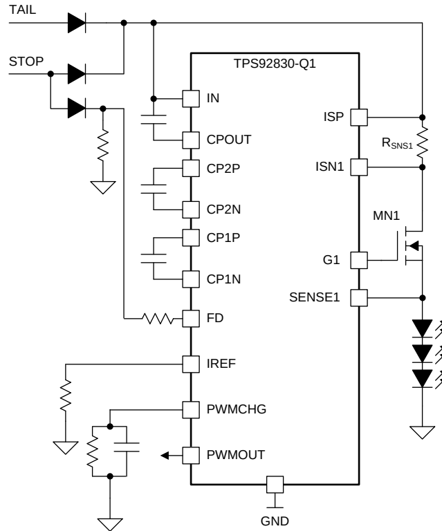
FIG 23. PWM Generator Dual-Brightness Configuration
