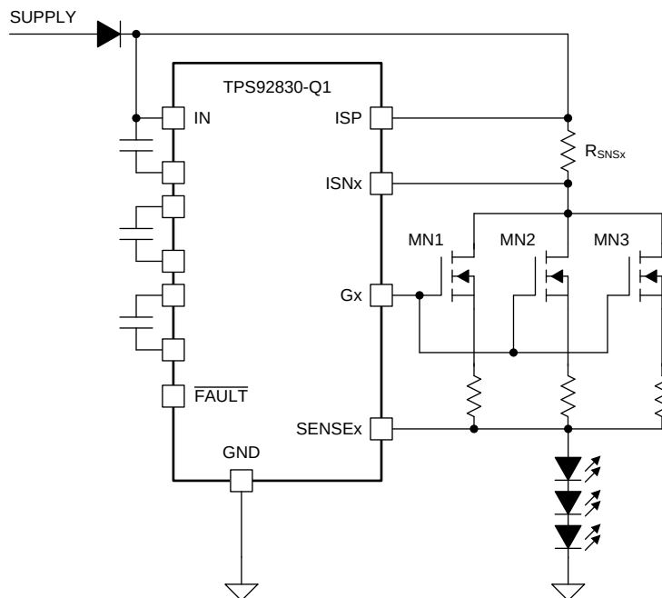
FIG 22. Parallel MOSFET Driving
