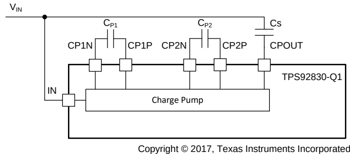
Figure 20. Charge Pump
