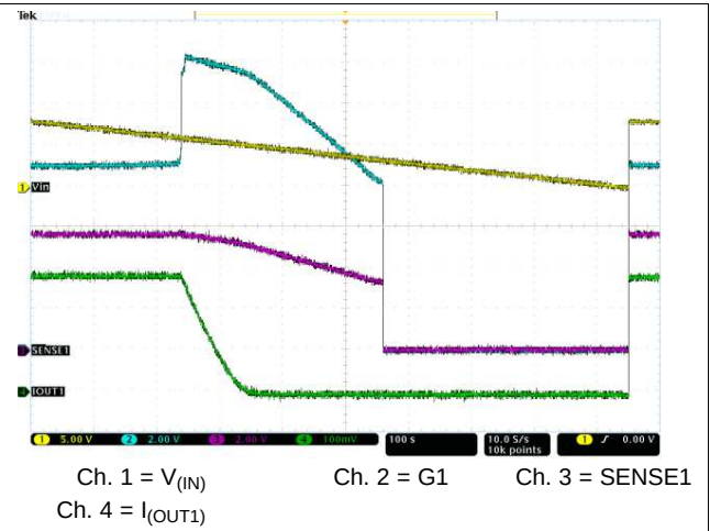
FIG 15. Slow Decrease, Quick Increase of Supply Voltage
