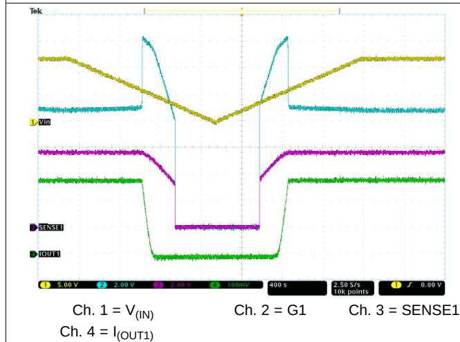
FIG 16. Slow Decrease and Slow Increase of Supply Voltage
