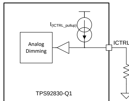
FIG 27. Internal High-Precision Pullup Current Source
