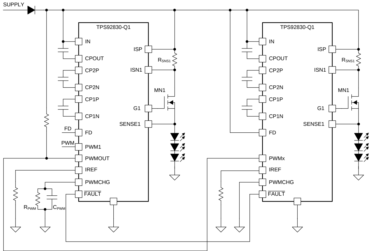
图 33. PWM Generator Master-Slave Configuration
