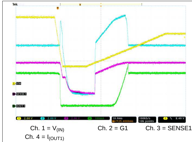
FIG 14. Fast Power Down and Slow Power Up
