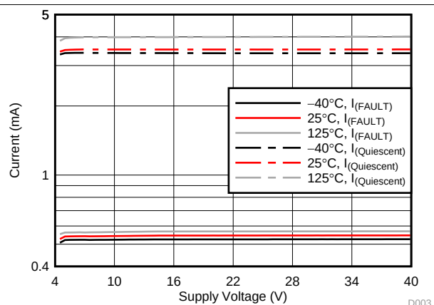
Figure 5. Device Current vs Supply Voltage
