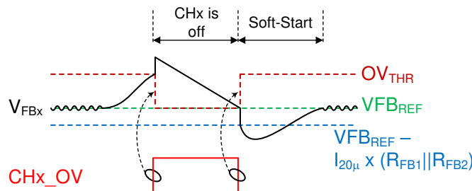
FIG 7-16. Non-latched OV Fault in CV Mode
