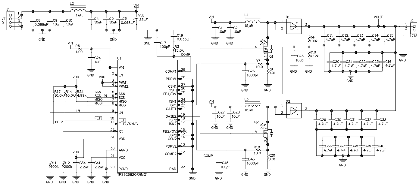
图 8-24. CV Mode Two-Phase BOOST
