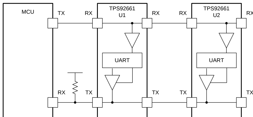
Figure 27. Communications Connections
