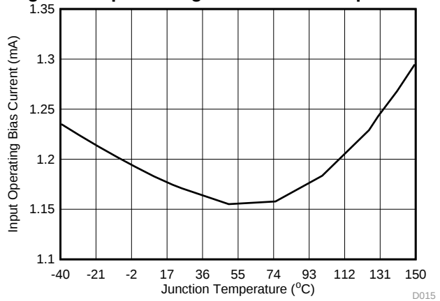
V_{\text{VIN}} = 5.5 \text{ V} f_{\text{CLK}} = 8.57 \text{ MHz} Figure 2. Input Voltage Current vs Temperature
