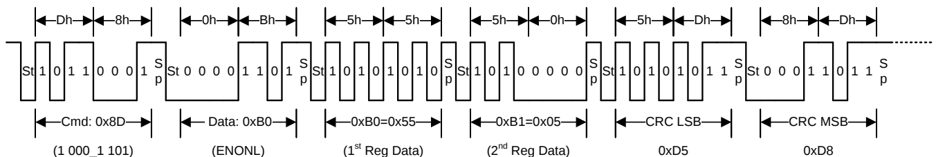
Figure 33. 2-Byte Write Example Waveform
