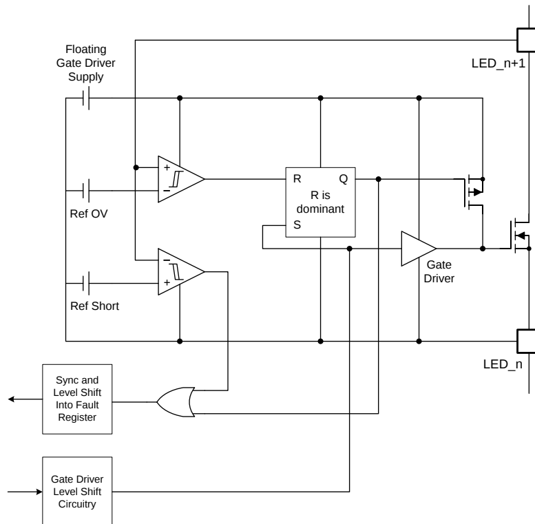
Figure 18. Fault Detection Block
