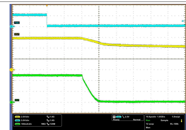
Figure 25. Output Current With PWM Input
