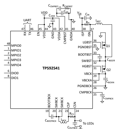
Simplified Schematic
