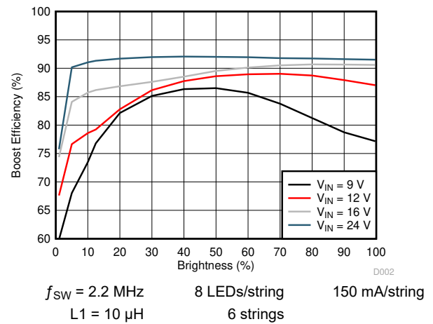
6-3. Boost Efficiency
