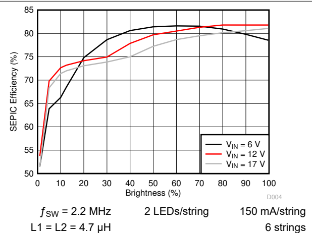
6-5. SEPIC Efficiency
