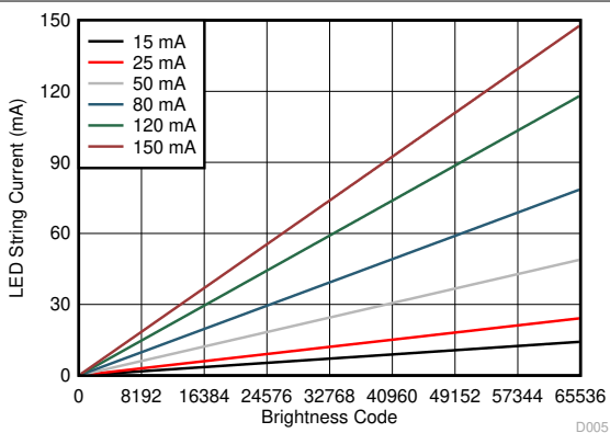
6-6. Current Linearity
