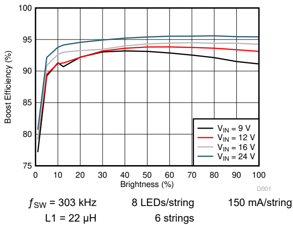
6-2. Boost Efficiency
