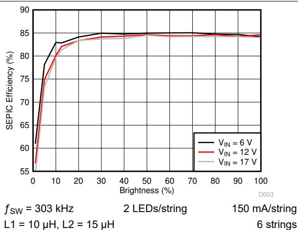
6-4. SEPIC Efficiency
