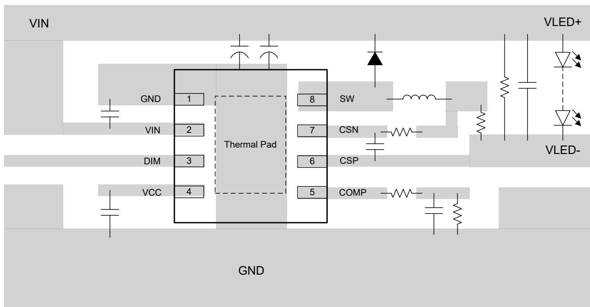
図 8-25. 8-Pin WSON Top View Layout Example
