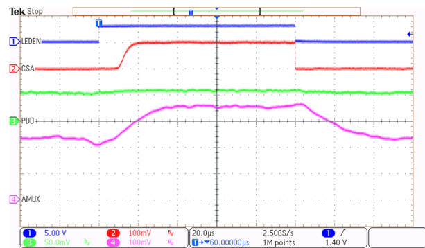
9-6. LED Driver and Photo Amplifier Waveforms
