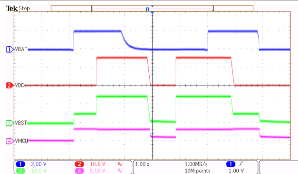
9-4. 15V AC/DC Supply with Battery Backup Handoff
