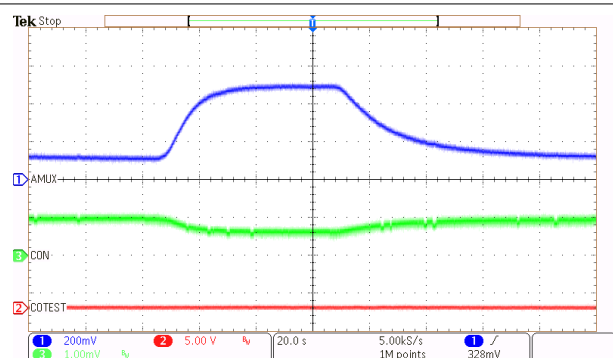
9-8. Carbon Monoxide Amplifier Waveforms with Calibration Gas
