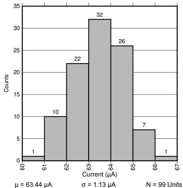
6-2. Bias Block Current
