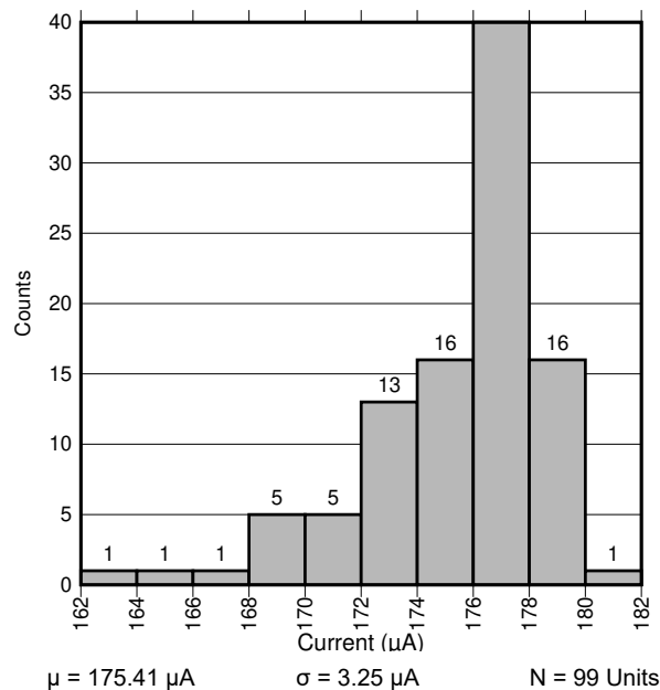
6-1. 8 MHz Oscillator Current
