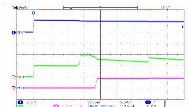
图 9-2. Power-up Waveforms
