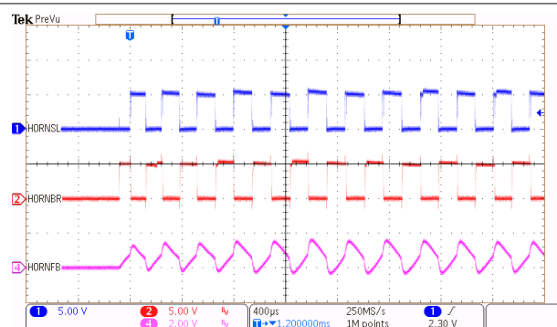
9-9. 3-Terminal Horn Driver Waveforms
