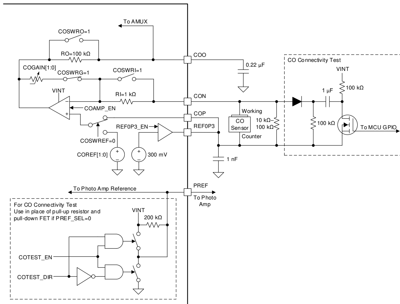
8-6. Carbon Monoxide Detection Circuit Referenced to 300mV
