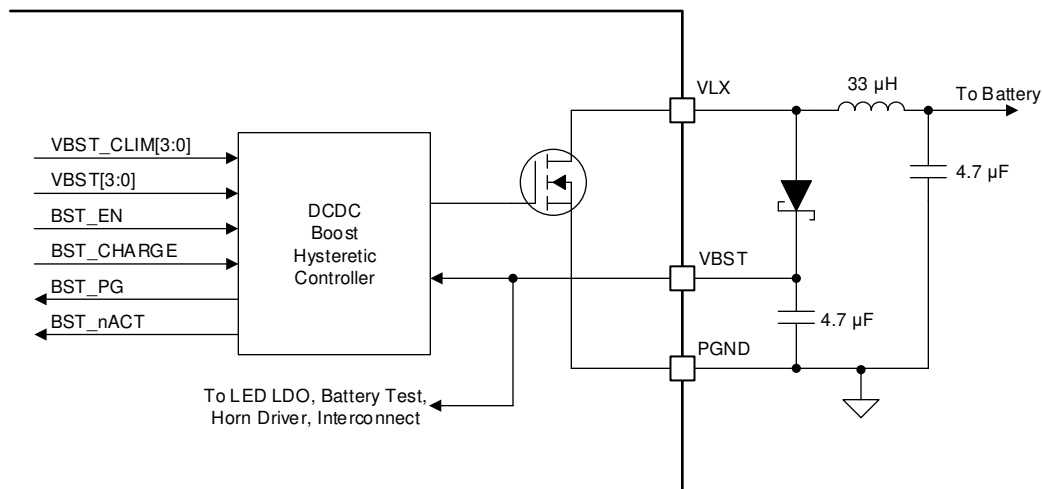
FIG 8-7. DC to DC Hysteretic Boost Circuit
