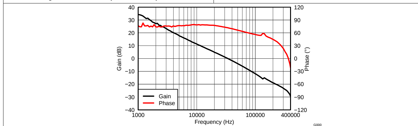
Figure 10. V OUT = 1.8 V, I OUT = 6 A, C OUT1 = 200 µF ceramic, f SW = 480 kHz
