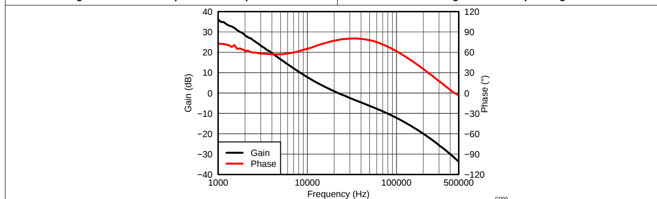
Figure 10. V OUT = 1.8 V, I OUT = 6 A, C OUT1 = 47 µF ceramic, C OUT2 = 100 µF POSCAP, f SW = 1 MHz
