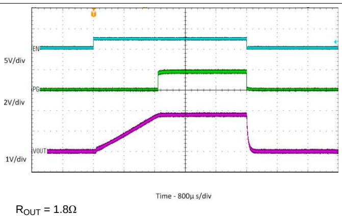
图 29. Startup / Shutdown with Resistance Load
