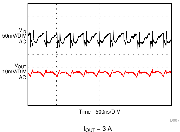
8-19. Input and Output Ripple in PWM Mode
