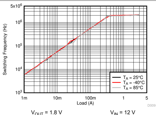
8-17. Switching Frequency
