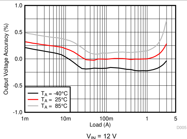
8-15. Load Regulation
