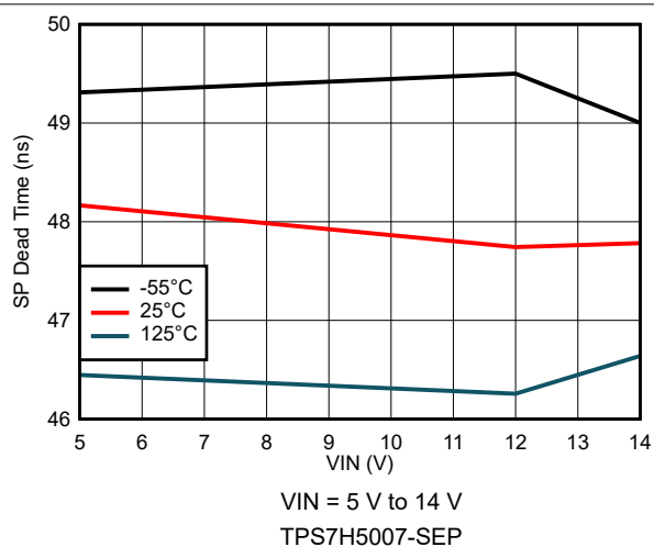
7-56. SP Dead Time Variation
