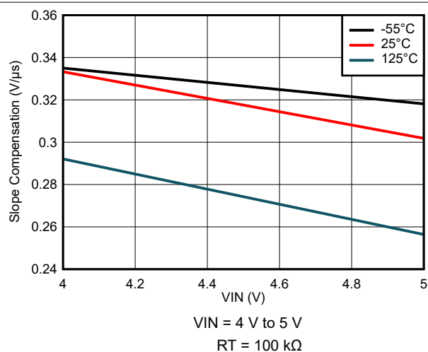
7-69. Slope Compensation Variation
