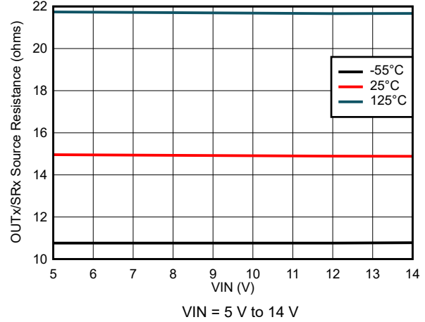
FIG 7-62. Output Source Resistance Variation
