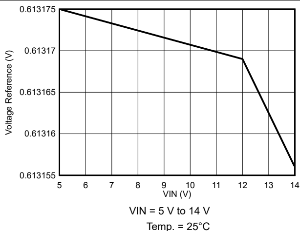
7-14. Voltage Reference Variation
