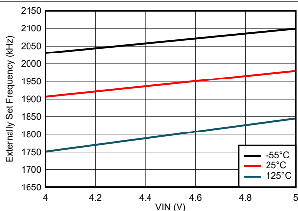
7-25. Externally Set Frequency Variation
