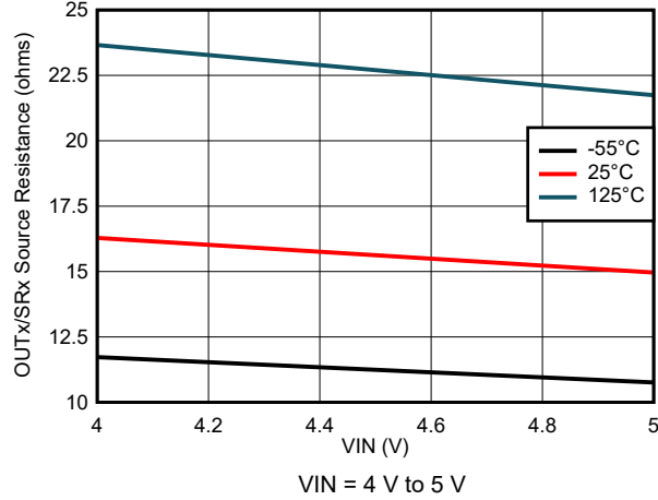
FIG 7-61. Output Source Resistance Variation
