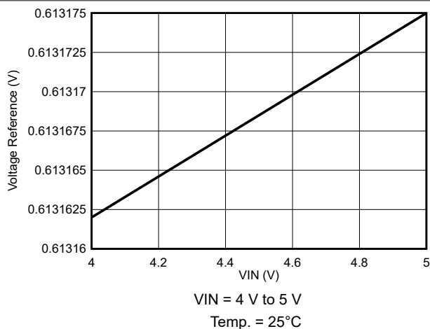
7-13. Voltage Reference Variation
