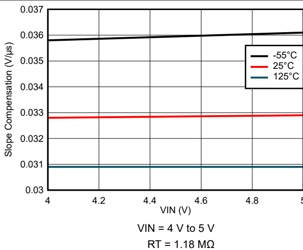
FIG 7-65. Slope Compensation Variation
