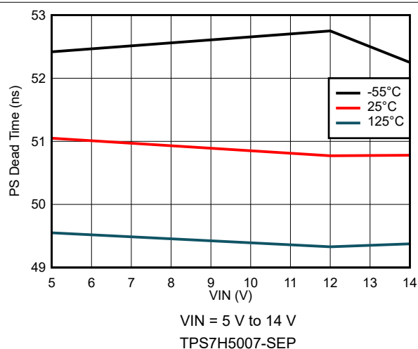
7-48. PS Dead Time Variation
