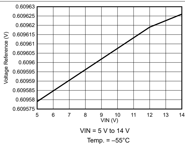
7-12. Voltage Reference Variation
