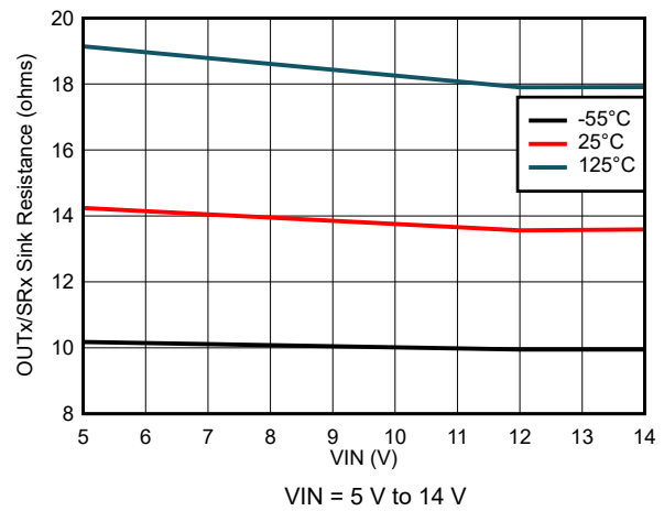
FIG 7-64. Output Sink Resistance Variation
