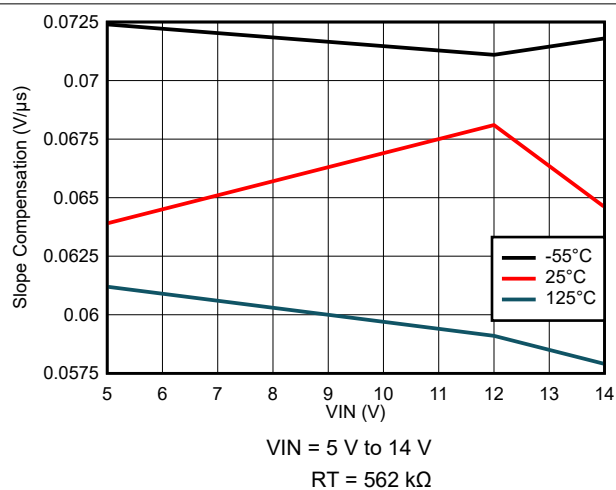
7-68. Slope Compensation Variation
