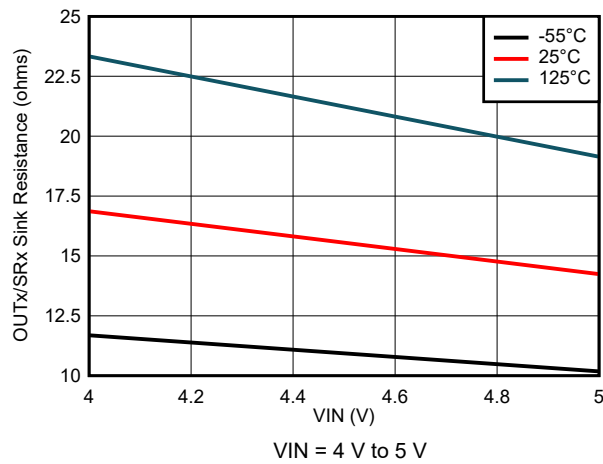
FIG 7-63. Output Sink Resistance Variation
