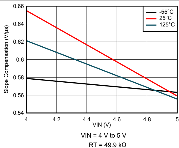
7-71. Slope Compensation Variation
