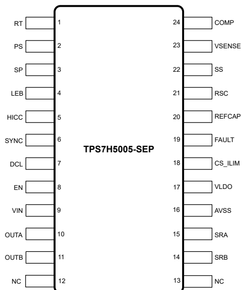
6-1. TPS7H5005-SEP PW Package 24-Pin TSSOP (Top View)
