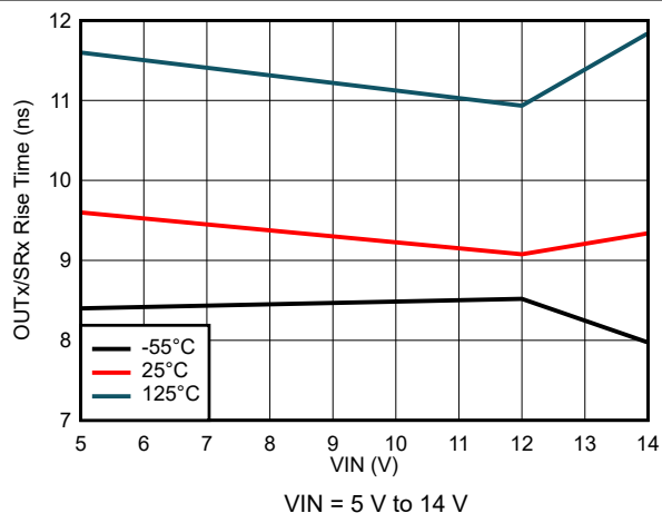
7-58. Output Rise Time Variation
