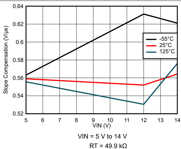
7-72. Slope Compensation Variation
