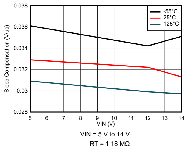
FIG 7-66. Slope Compensation Variation
