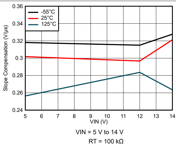
7-70. Slope Compensation Variation
