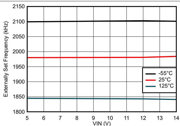
7-26. Externally Set Frequency Variation
