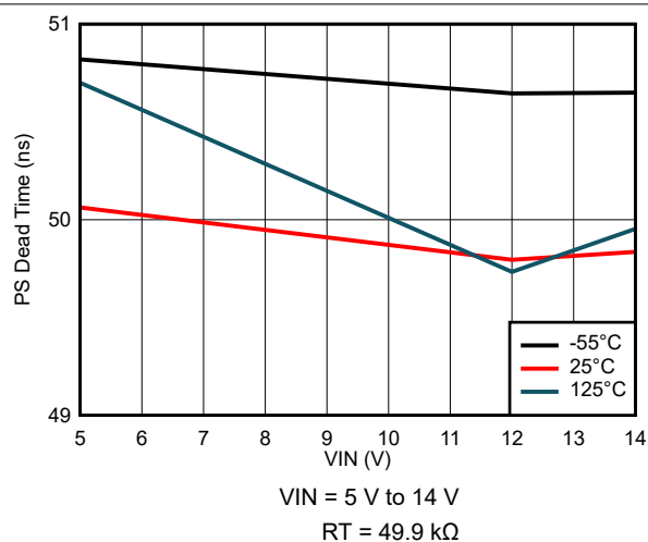
7-44. PS Dead Time Variation
