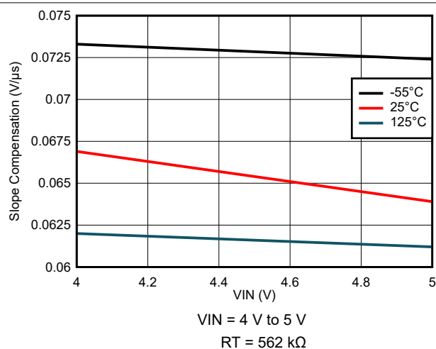
7-67. Slope Compensation Variation
