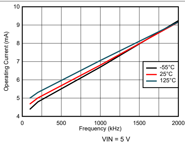
図 7-1. Operating Current Variation
