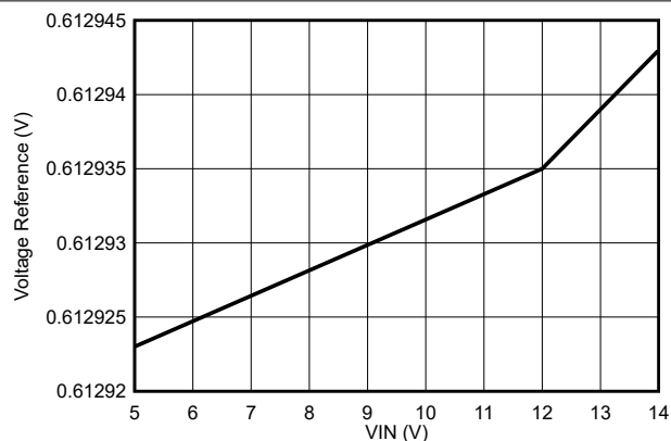
図 7-14. Voltage Reference Variation
