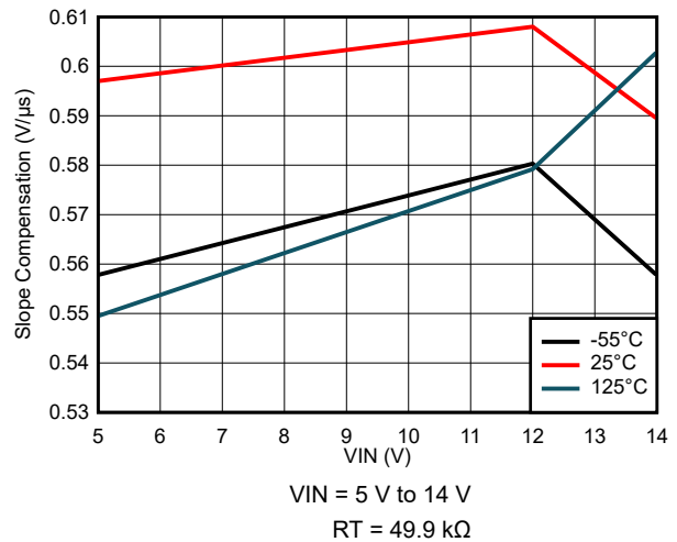
Figure 7-72. Slope Compensation Variation
