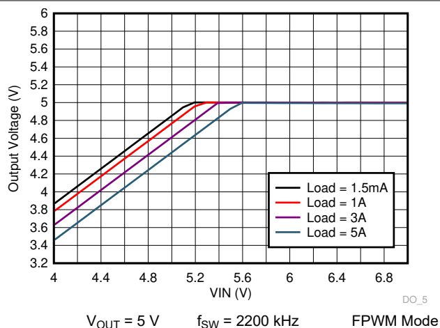
8-12. TPS7H4010-SEP Dropout Curve
