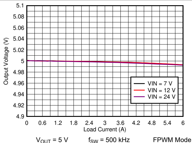
8-10. TPS7H4010-SEP Load and Line Regulation
