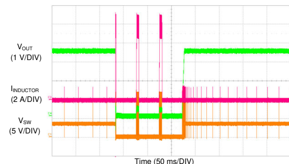
FIG 8-22. TPS7H4010-SEP Switching Waveform at Dropout
