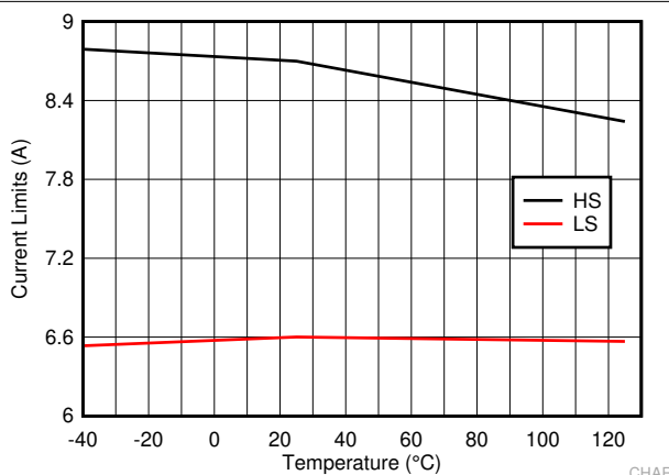
FIG 6-5. TPS7H4010-SEP High-Side and Low-Side Current Limit
