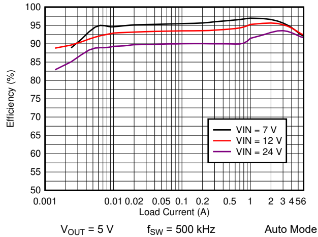
8-3. TPS7H4010-SEP Efficiency
