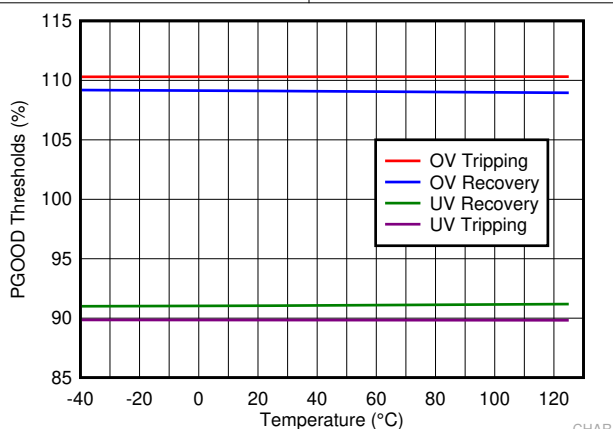
FIG 6-9. PGOOD Thresholds
