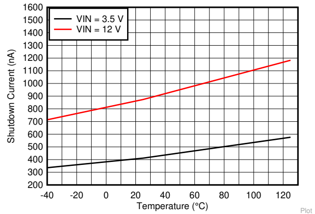
FIG 6-2. Shutdown Quiescent Current
