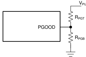
FIG 7-15. Divider for PGOOD Pullup Voltage
