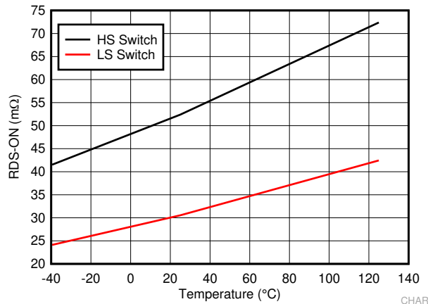
FIG 6-1. High-Side and Low-Side Switches R_{DS-ON}
