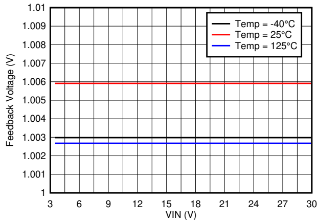
FIG 6-3. Feedback Voltage
