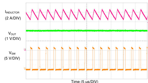
FIG 8-21. TPS7H4010-SEP Switching Waveform and V_{OUT} Ripple
