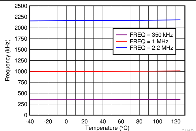
FIG 6-6. Switching Frequency Set by R_T Resistor
