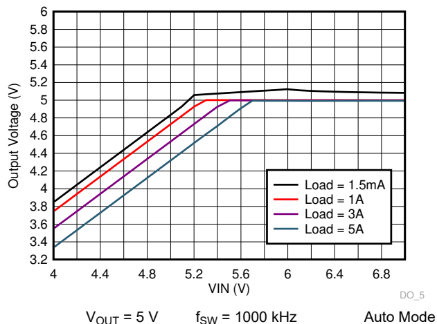
8-14. TPS7H4010-SEP Dropout Curve
