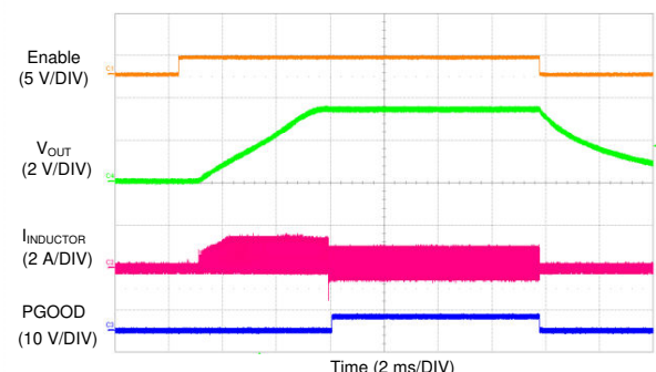
FIG 8-23. TPS7H4010-SEP Overcurrent Behavior
