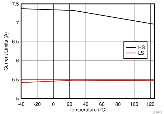
FIG 6-4. TPS7H4010-SEP High-Side and Low-Side Current Limits
