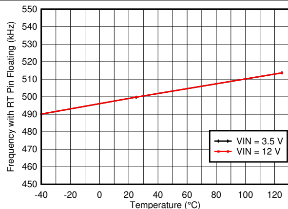
FIG 6-7. Switching Frequency With RT Pin Open Circuit
