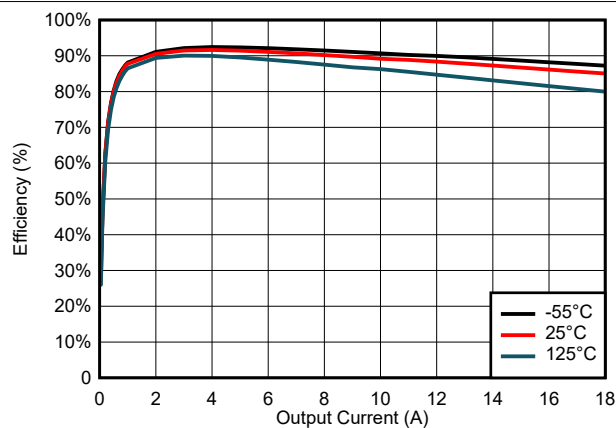
FIG 6-31. Efficiency for VIN = 7 V
