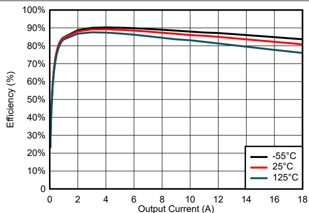
FIG 6-32. Efficiency for VIN = 7 V
