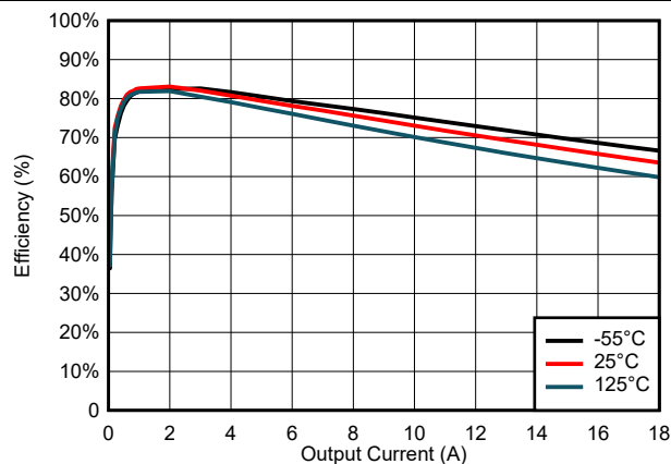
FIG 6-33. Efficiency for VIN = 7 V
