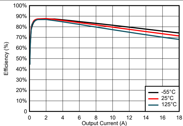
FIG 6-34. Efficiency for VIN = 7 V
