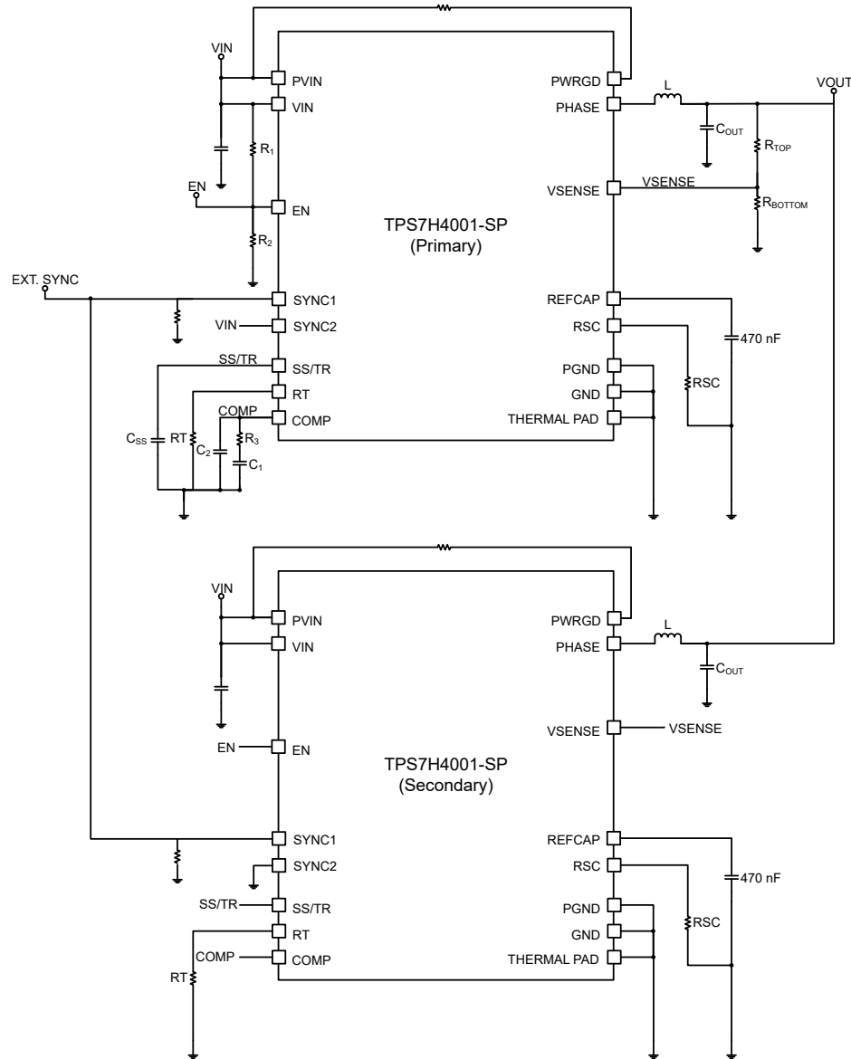
図 9-3. Parallel Configuration With External Sync
