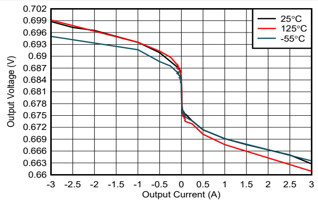
VDD = 3.6 V VDDQSNS = 1.35 V 6-4. Output Voltage vs Output Current
