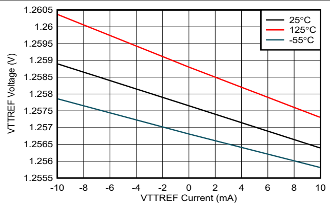
VDDQSNS = 2.5 V 6-6. VTTREF Voltage vs VTTREF Current
