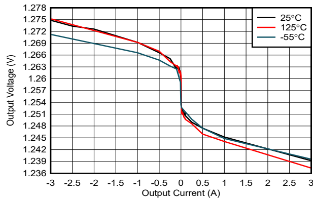
VDD = 3.6 V VDDQSNS = 2.5 6-1. Output Voltage vs Output Current
