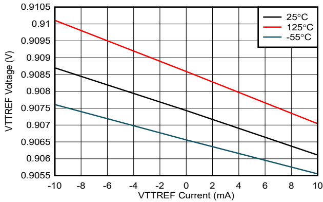
Figure 6-7. VTTREF Voltage vs VTTREF Current
