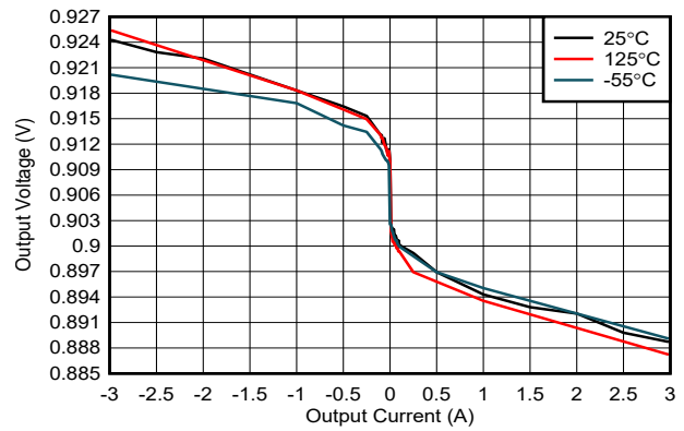
VDD = 3.6 V VDDQSNS = 1.8 V 6-2. Output Voltage vs Output Current
