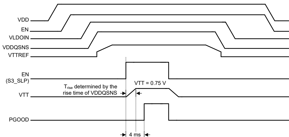
図 8-4. Typical Timing Diagram of Tracking Startup and Shutdown
