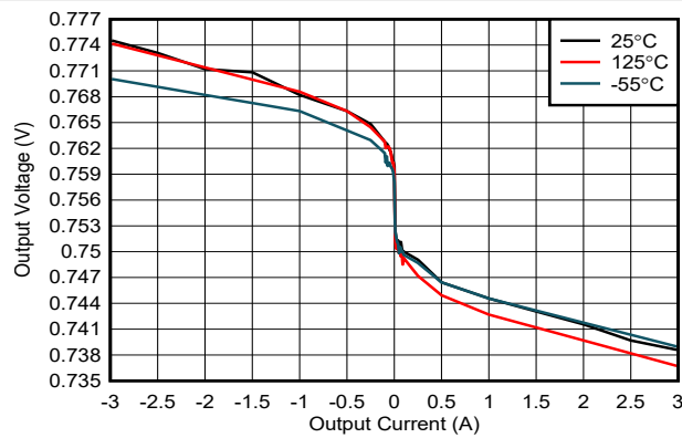
VDD = 3.6 V VDDQSNS = 1.5 V 6-3. Output Voltage vs Output Current
