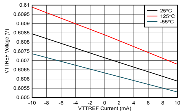
Figure 6-10. VTTREF Voltage vs VTTREF Current
