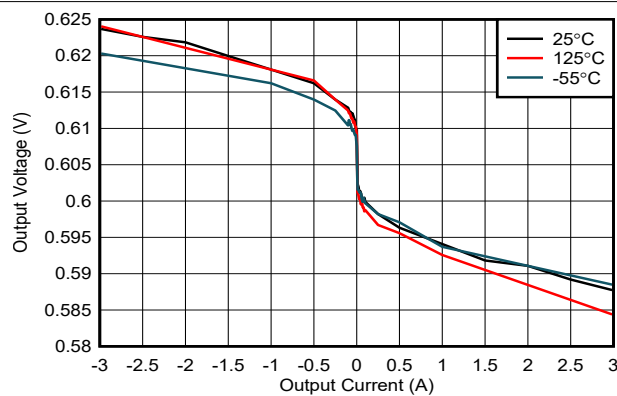
VDD = 3.6 V VDDQSNS = 1.2 V 6-5. Output Voltage vs Output Current
