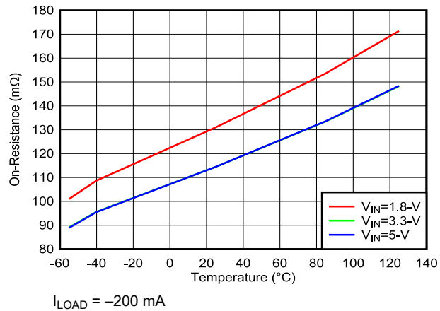
6-5. On-Resistance vs Junction Temperature
