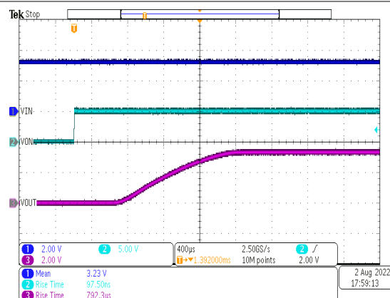
6-21. Rise Time with V_{IN} = 3.3 V
