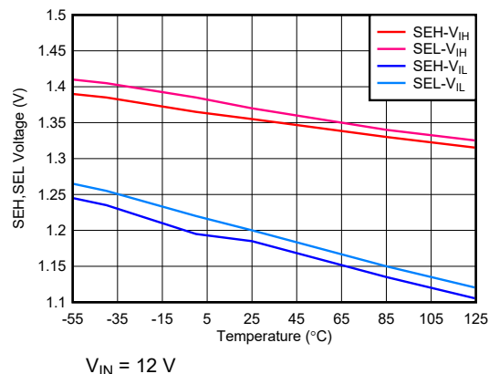
Figure 6-4. SEH,SEL Voltage Threshold
