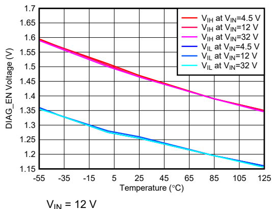
Figure 6-3. DIAG_EN Voltage Threshold
