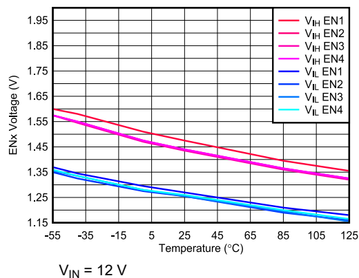
Figure 6-1. ENx Voltage Threshold
