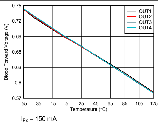
Figure 6-6. Body-Diode Forward Voltage
