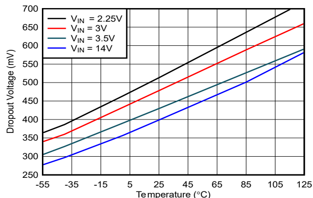
図 6-2. Dropout Voltage vs Temperature
