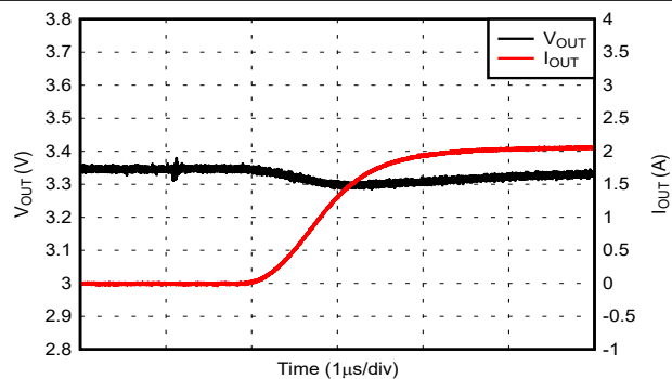
図 6-23. Load Step: 0A to 2A with V_{IN} = 5V
