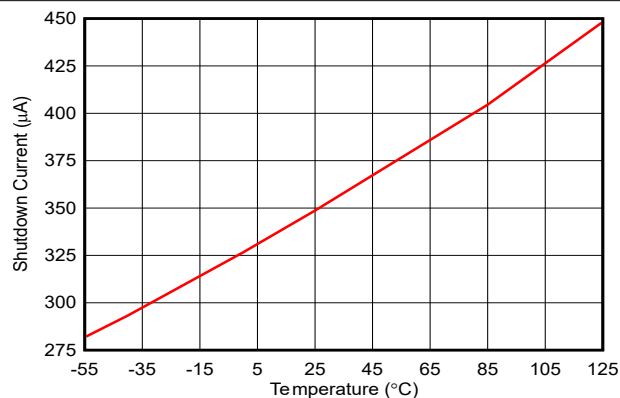
図 6-9. Shutdown Current vs Temperature
