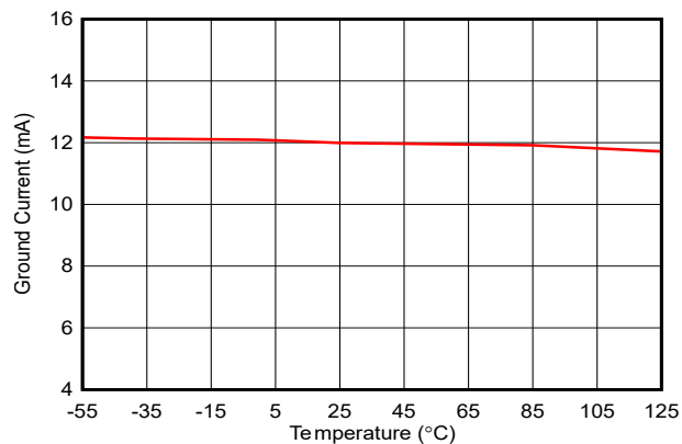
図 6-8. Ground Current vs Temperature
