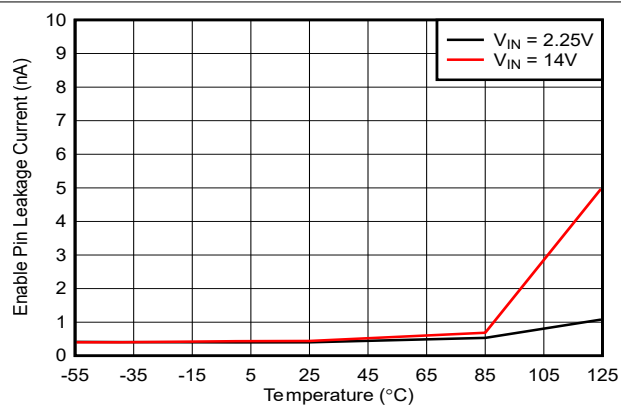
図 6-12. Enable Pin Leakage Current vs Temperature
