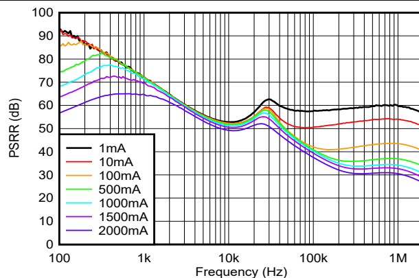
図 6-21. PSRR vs Frequency Across Current
