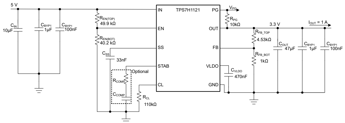
図 9-1. Application Schematic
