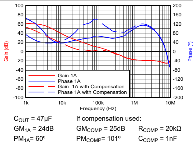
図 6-17. Gain and Phase Margins vs Frequency (Bode Plot)
