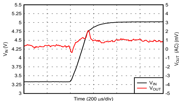
図 6-25. Line Step: 3.3V to 5V With I_{OUT} = 1.8A
