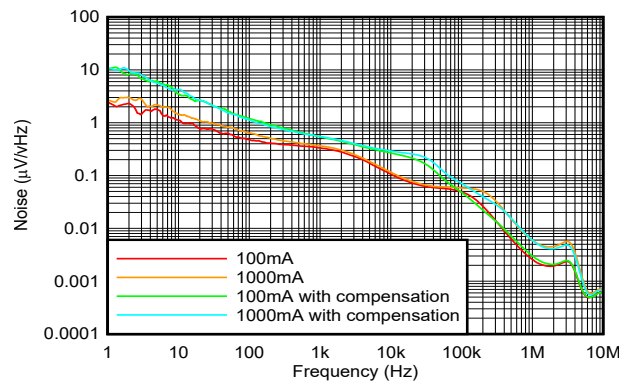
図 6-20. Output Noise vs Frequency, External Compensation Comparison (Noise Spectral Density)
