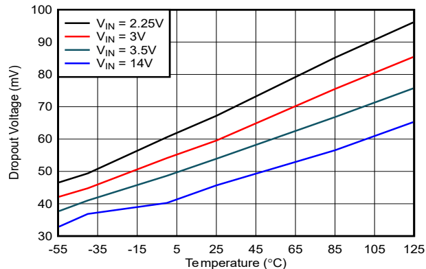
図 6-4. Dropout Voltage vs Temperature
