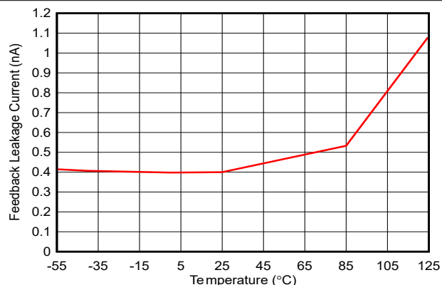
図 6-10. Feedback Pin Leakage Current vs Temperature
