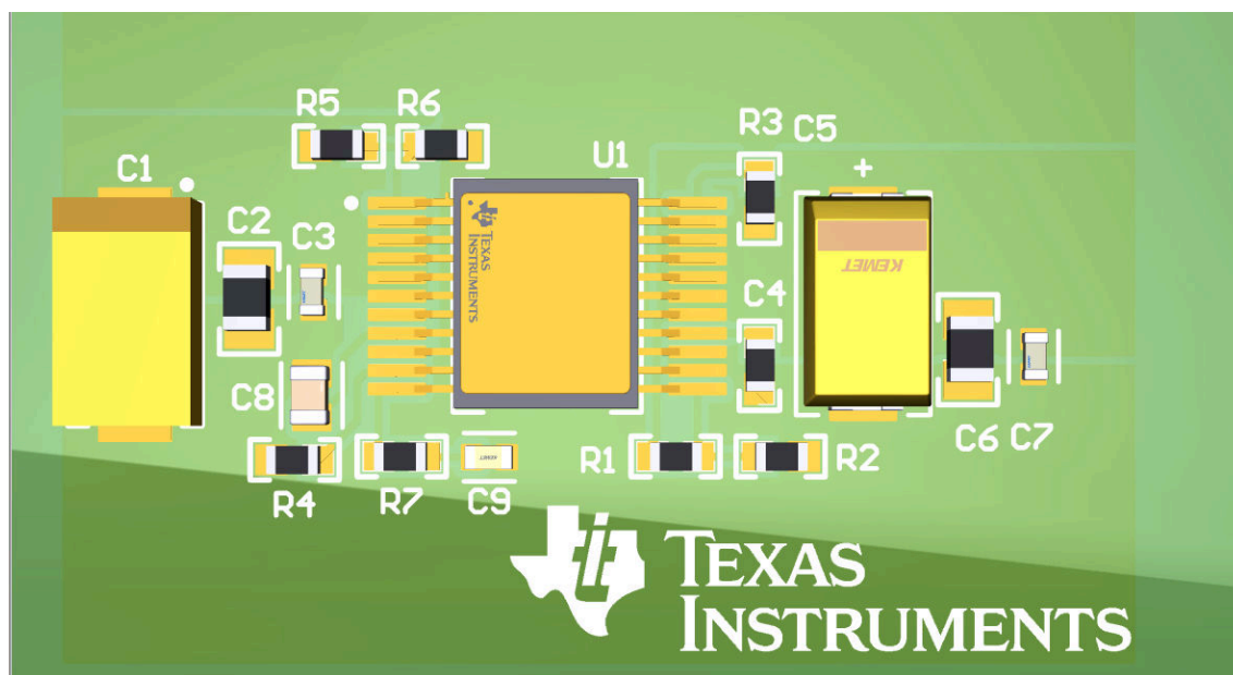
図 9-5. Printed Circuit Board Layout Example: 3D View
