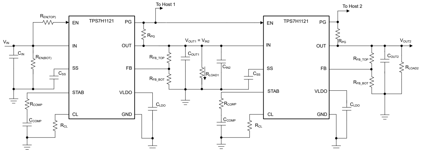
図 8-1. Sequenced Power Good
