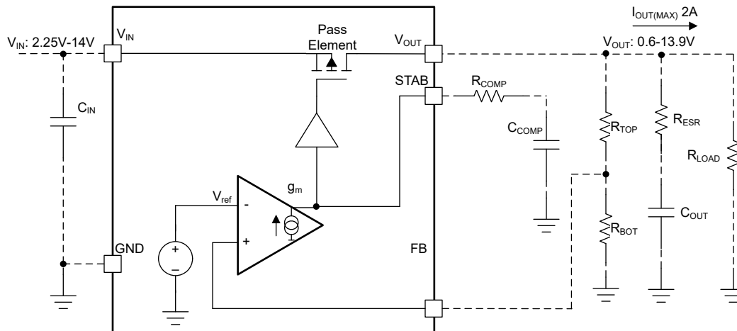
図 8-2. Simplified Compensation Schematic
