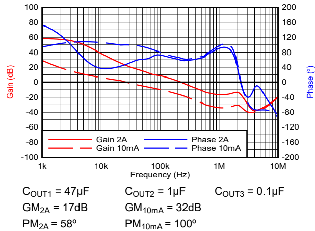
図 6-15. Gain and Phase Margin vs Frequency (Bode Plot)
