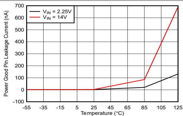
図 6-11. Power Good Pin Leakage Current vs Temperature
