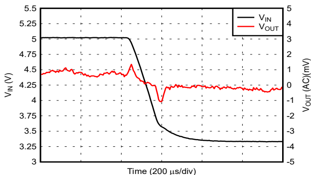
図 6-26. Line Step: 5V to 3.3V With I_{OUT} = 1.8A
