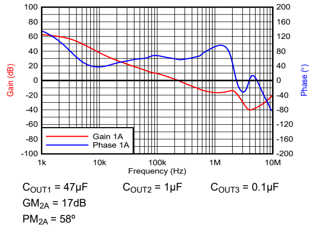
図 6-16. Gain and Phase Margin vs Frequency (Bode Plot)
