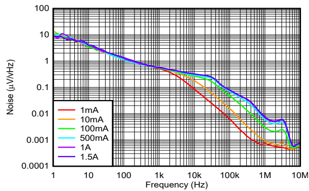
図 6-19. Output Noise vs Frequency Across Current (Noise Spectral Density)
