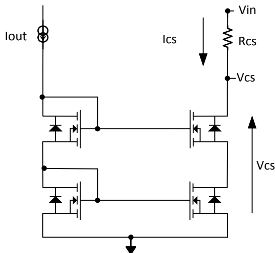
FIG 12. Cascode NMOS Current Mirror
