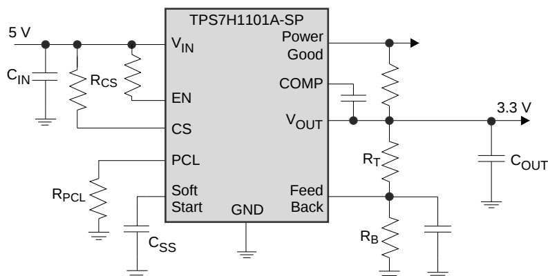
図 10. Typical Application Circuit
