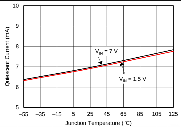
FIG 2. Quiescent Current vs Temperature
