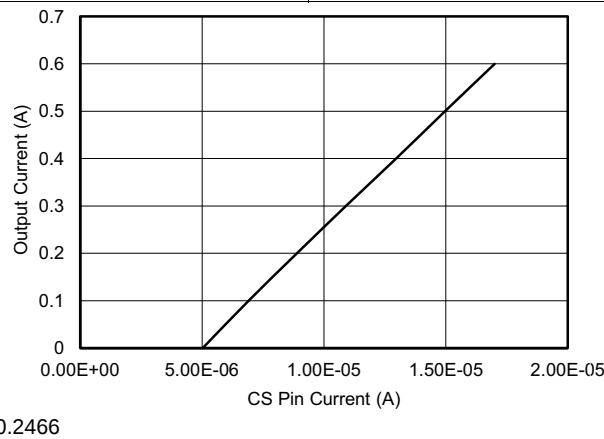
Figure 15. I_{OUT} (A) vs I_{CS} (A)
