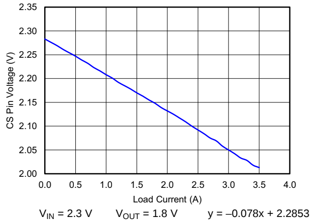
Figure 13. V_{CS} (V) vs I_{OUT} (A)
