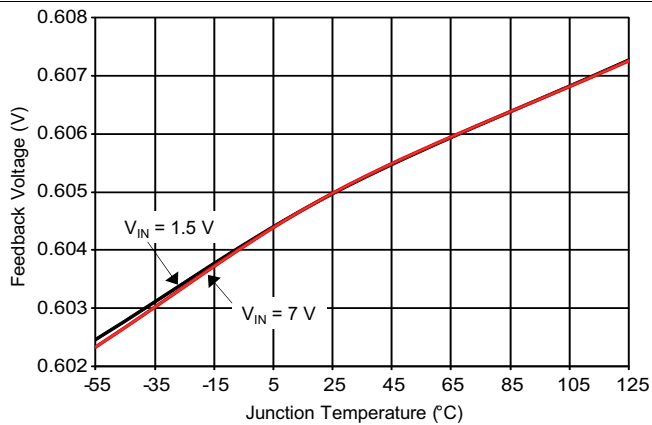
FIG 1. Feedback Voltage vs Temperature
