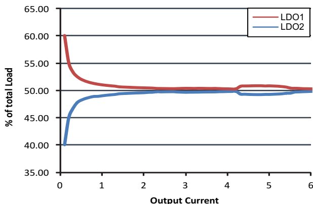
Figure 19. LDO Current Share
