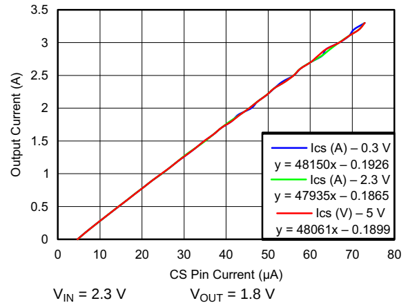
Figure 14. I_{OUT} (A) vs I_{CS} (A)
