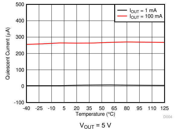
Figure 6-4. Quiescent Current vs Ambient Temperature
