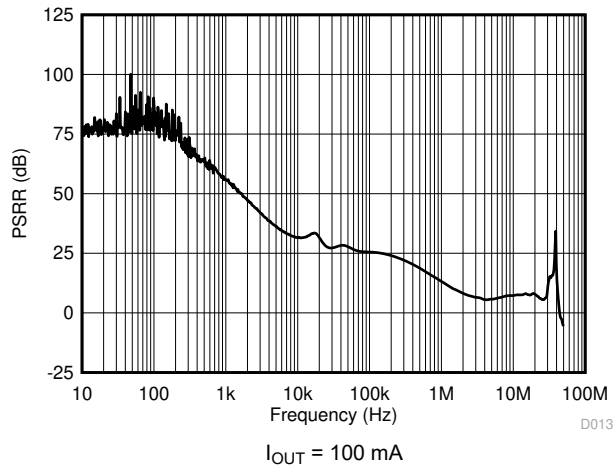
6-13. PSRR vs Frequency
