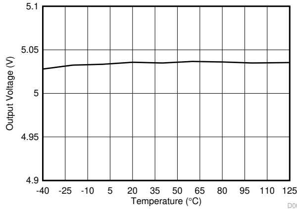
6-7. Output Voltage vs Ambient Temperature
