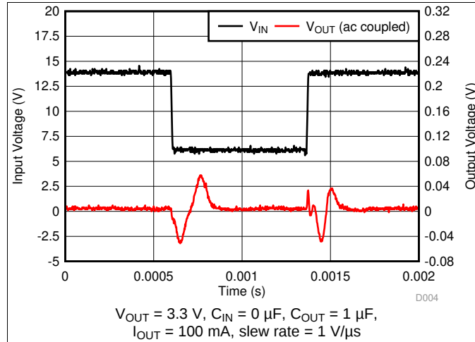
Figure 19. Line Transient
