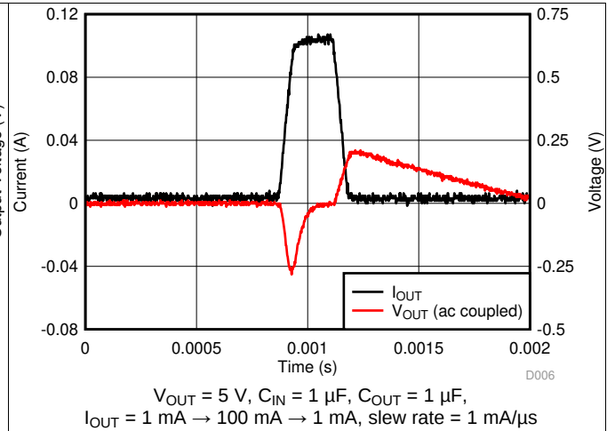
Figure 20. Load Transient
