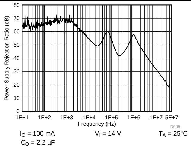
Figure 10. Power Supply Rejection Ratio
