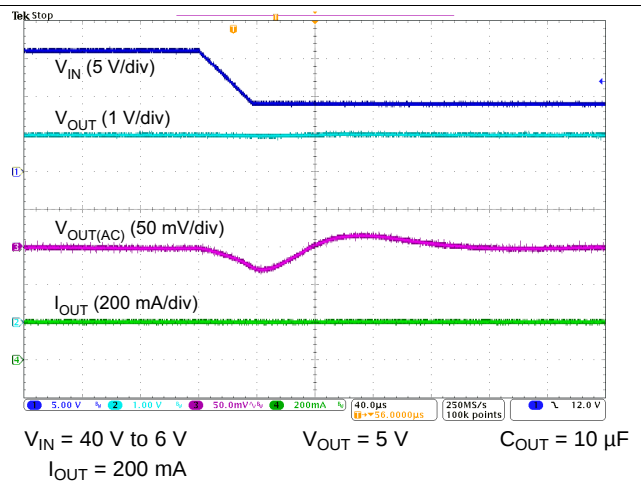
FIG 18. Line Transient
