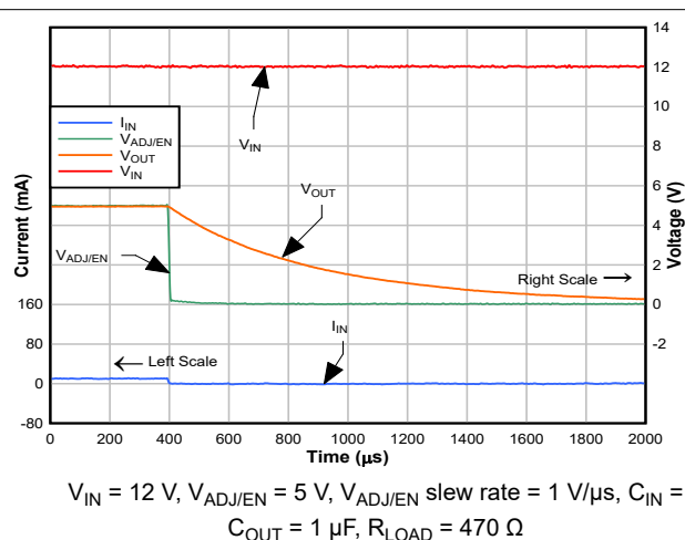
8-3. Power-Down
