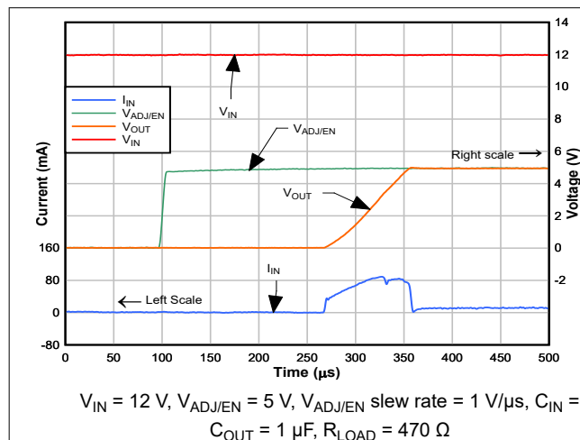
8-2. Power-Up
