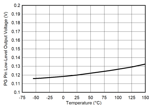
FIG 6-68. V_{PG} Low-Level Output Voltage vs Temperature
