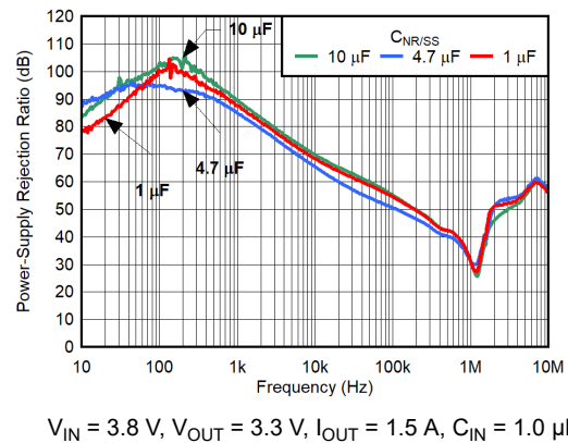
FIG 6-10. PSRR vs Frequency and C_{NR/SS}
