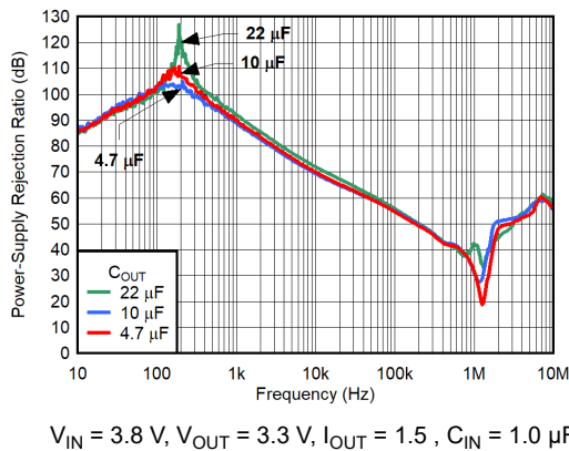
FIG 6-11. PSRR vs Frequency and C_{OUT}
