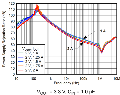
FIG 6-9. PSRR vs Frequency for Operating Headroom ( V_{OpHr} ) and I_{OUT}
