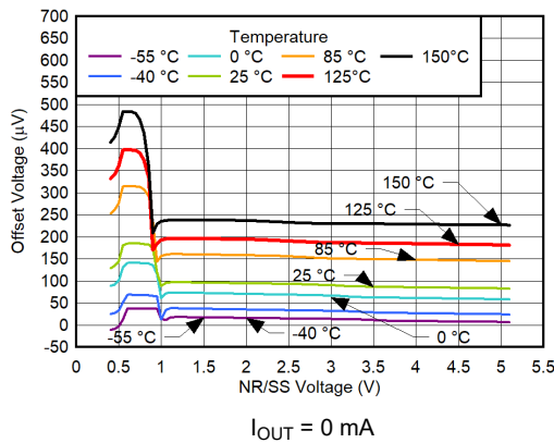
6-39. V_{OS} vs V_{NR/SS} and Temperature for I_{OUT} = 0\text{ mA}
