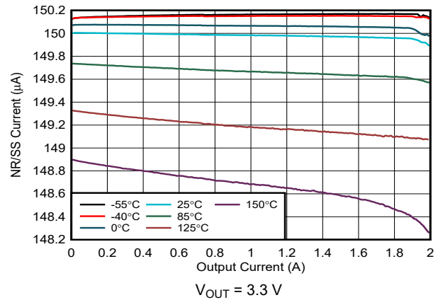
6-40. I_{NR/SS} vs I_{OUT} and Temperature for V_{IN} = 3.8\text{ V}
