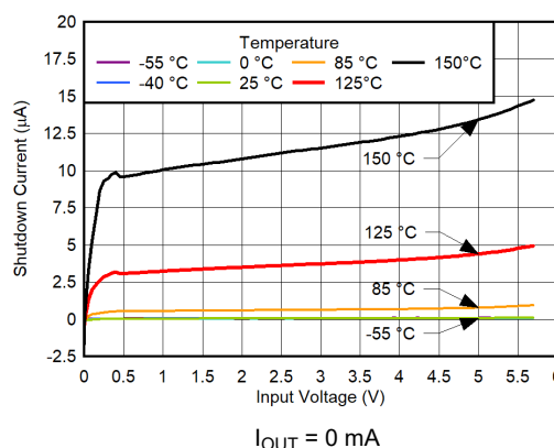
FIG 6-72. Shutdown Current vs V_{IN} and Temperature
