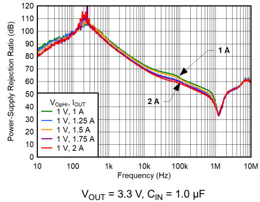
FIG 6-8. PSRR vs Frequency for Operating Headroom ( V_{OpHr} ) and I_{OUT}
