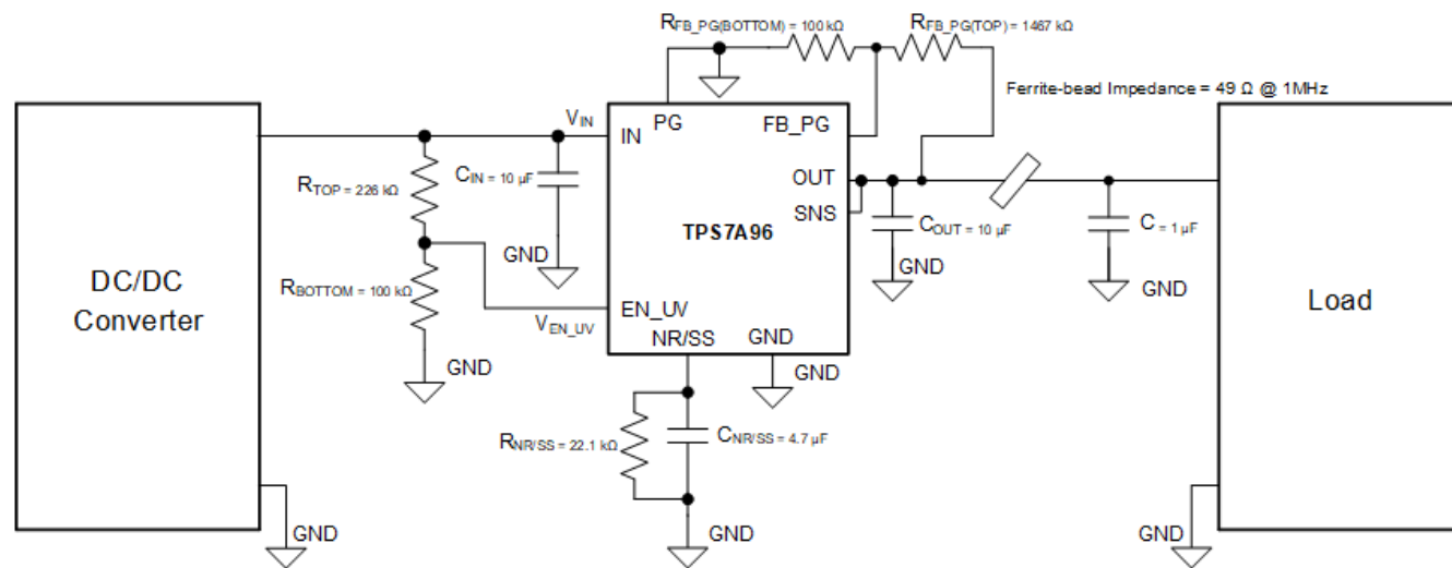
8-27. Typical Application Circuit With Added Pi-Filter
