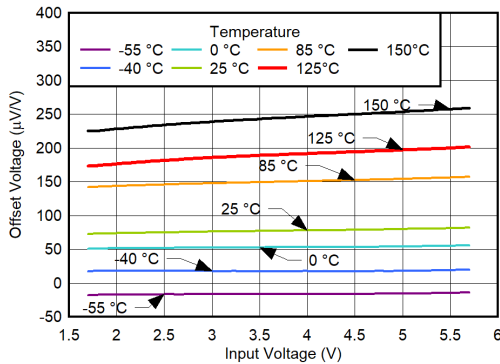
FIG 6-45. V_{OS} vs V_{IN} and Temperature for V_{OUT} = 1.8\text{ V}
