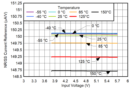
FIG 6-46. I_{NR/SS} vs V_{IN} and Temperature for V_{OUT} = 3.3\text{ V}
