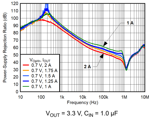
FIG 6-7. PSRR vs Frequency for Operating Headroom ( V_{OpHr} ) and I_{OUT}
