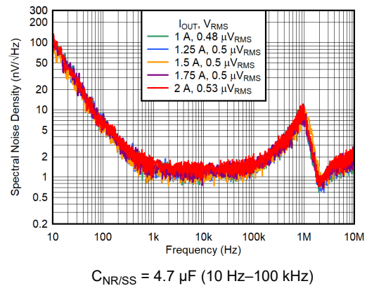
FIG 6-12. Output Voltage Noise Density vs Frequency for I_{OUT} and V_{OUT} = 1.2\text{ V}
