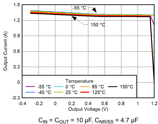
FIG 6-83. 100% Current Limit vs Temperature for V_{OUT} = 1.2\text{ V}
