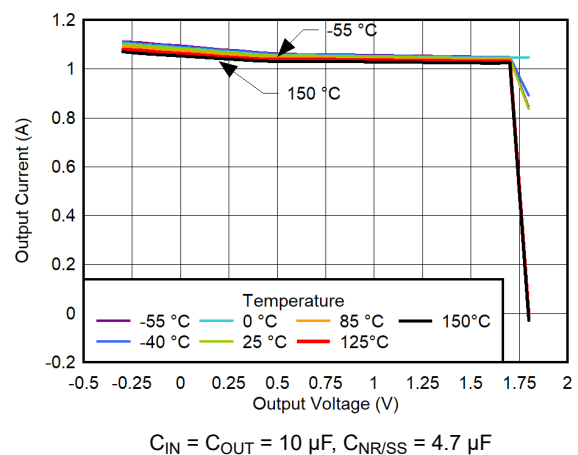
FIG 6-88. 80% Current Limit vs Temperature for V_{OUT} = 1.8\text{ V}
