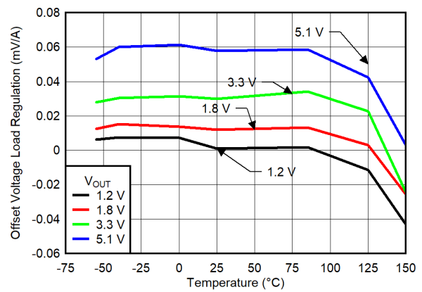
FIG 6-48. V_{OS} Load Regulation
