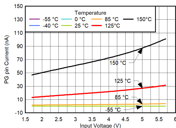
6-102. PG Pin Current vs V_{IN} and Temperature
