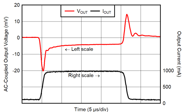
FIG 6-24. Load Transient Response for V_{OUT} = 1.2\text{ V} , I_{OUT} = 100\text{ mA} to 1\text{ A}
