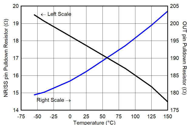
6-104. NR/SS and OUT Pulldown Resistors vs Temperature
