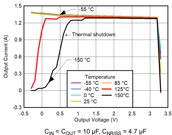
FIG 6-85. 100% Current Limit vs Temperature for V_{OUT} = 3.3\text{ V}
