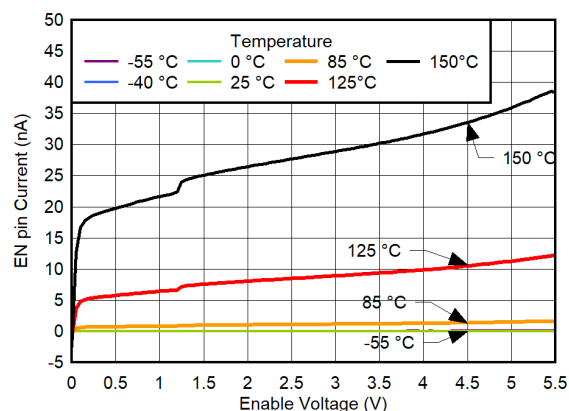
FIG 6-98. EN Pin Current vs Enable Voltage and Temperature for V_{IN} = 5.7\text{ V}
