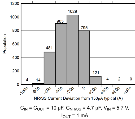
FIG 6-45. I_{NR/SS} Distribution
