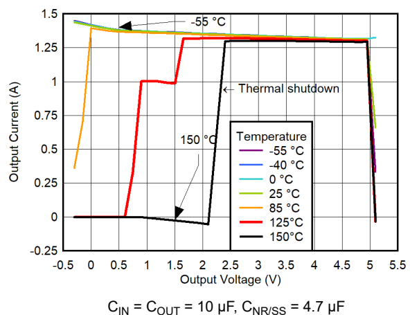
FIG 6-86. 100% Current Limit vs Temperature for V_{OUT} = 5.1\text{ V}
