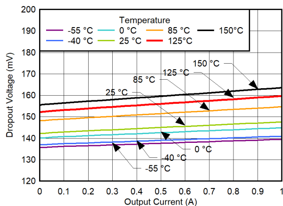
FIG 6-43. Dropout Voltage vs I_{OUT} for V_{OUT} = 3.3\text{ V}
