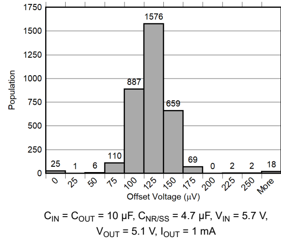
FIG 6-46. V_{OS} Distribution
