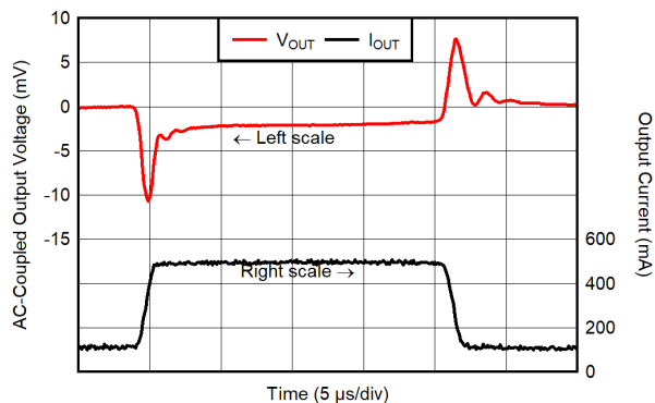
FIG 6-23. Load Transient Response for V_{OUT} = 1.2\text{ V} , I_{OUT} = 100\text{ mA} to 500\text{ mA}
