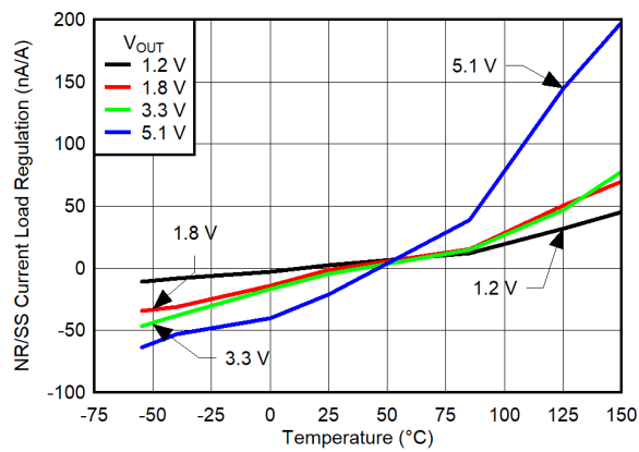
FIG 6-47. I_{NR/SS} Load Regulation
