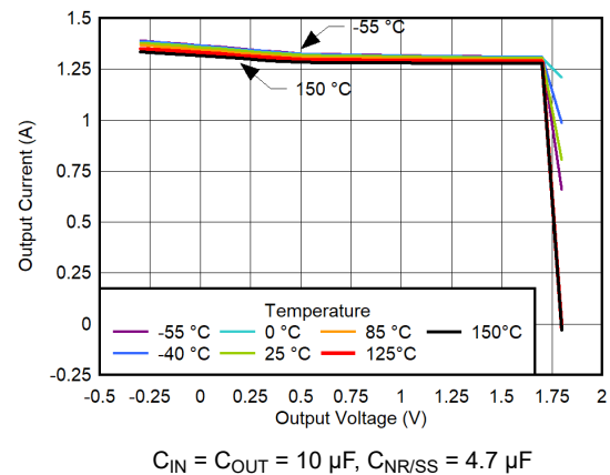
FIG 6-84. 100% Current Limit vs Temperature for V_{OUT} = 1.8\text{ V}
