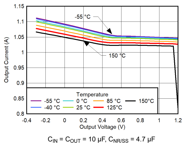
FIG 6-87. 80% Current Limit vs Temperature for V_{OUT} = 1.2\text{ V}
