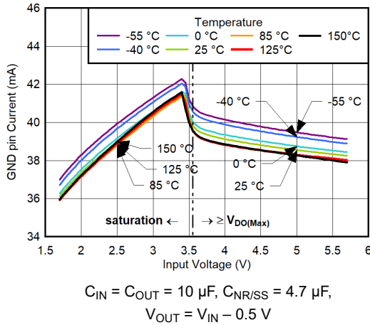
Figure 6-77. GND Pin Current vs V_{IN} and Temperature for I_{OUT} = 500 \text{ mA}
