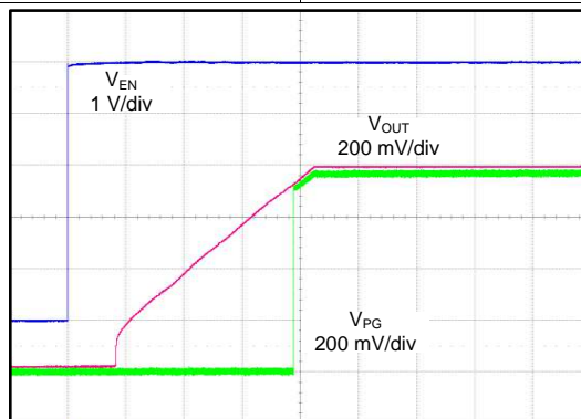
FIG 33. Start-Up ( SS\_CTRL = \text{GND} , C_{NR/SS} = 10\text{ nF} )
