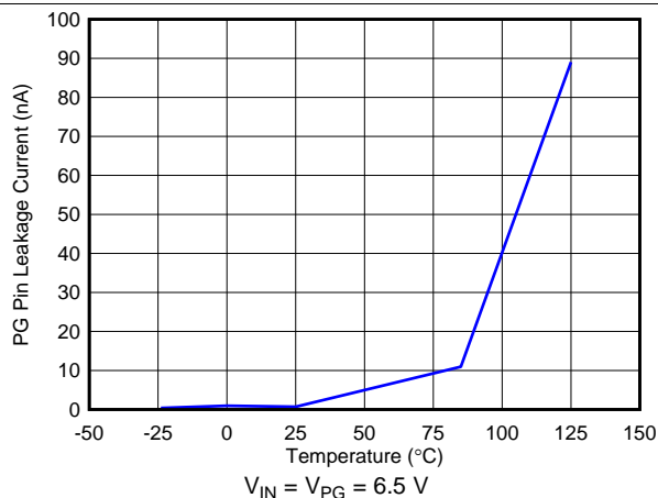
FIG 24. PG Leakage Current vs Temperature
