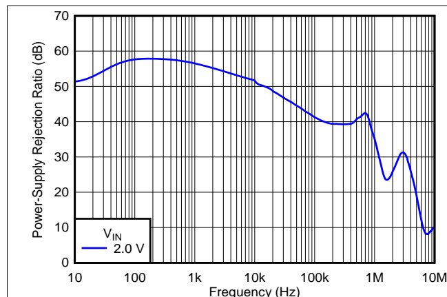
✎ 40. PSRR vs Frequency
