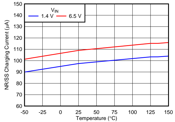
FIG 26. Soft-Start Current vs Temperature (SS_CTRL = V_{IN} )
