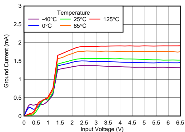
FIG 20. Ground Current vs Input Voltage
