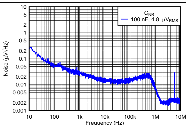
✎ 41. Output Noise vs Frequency
