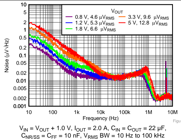
FIG 8. Spectral Noise Density vs Frequency and Output Voltage
