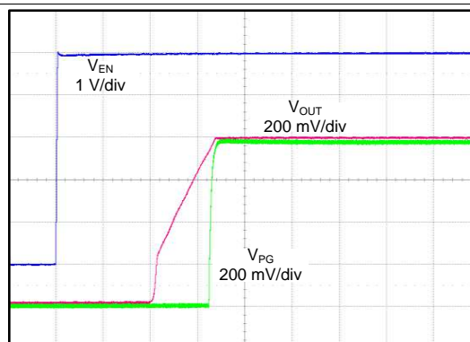
FIG 32. Start-Up ( SS\_CTRL = \text{GND} , C_{NR/SS} = 0\text{ nF} )
