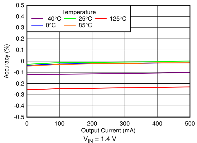
Figure 16. Load Regulation
