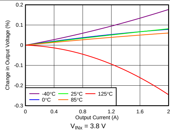
Figure 26. Load Regulation ( V_{\text{OUTX}} = 3.3\text{ V} )
