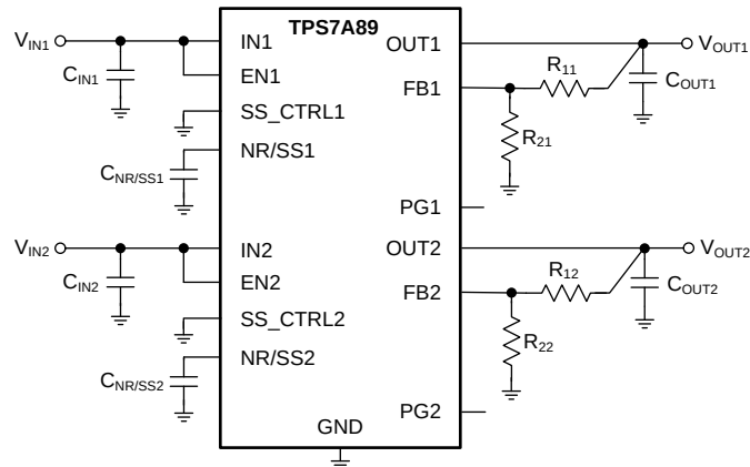
Figure 48. Adjustable Operation
