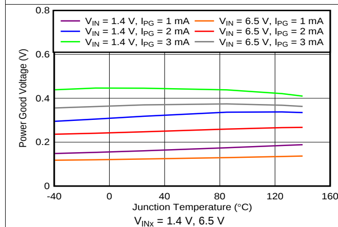
FIG 33. PG Low Level vs Temperature
