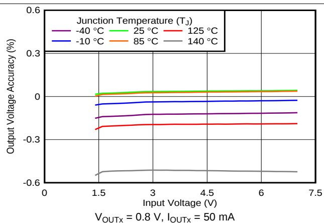
Figure 26. Line Regulation
