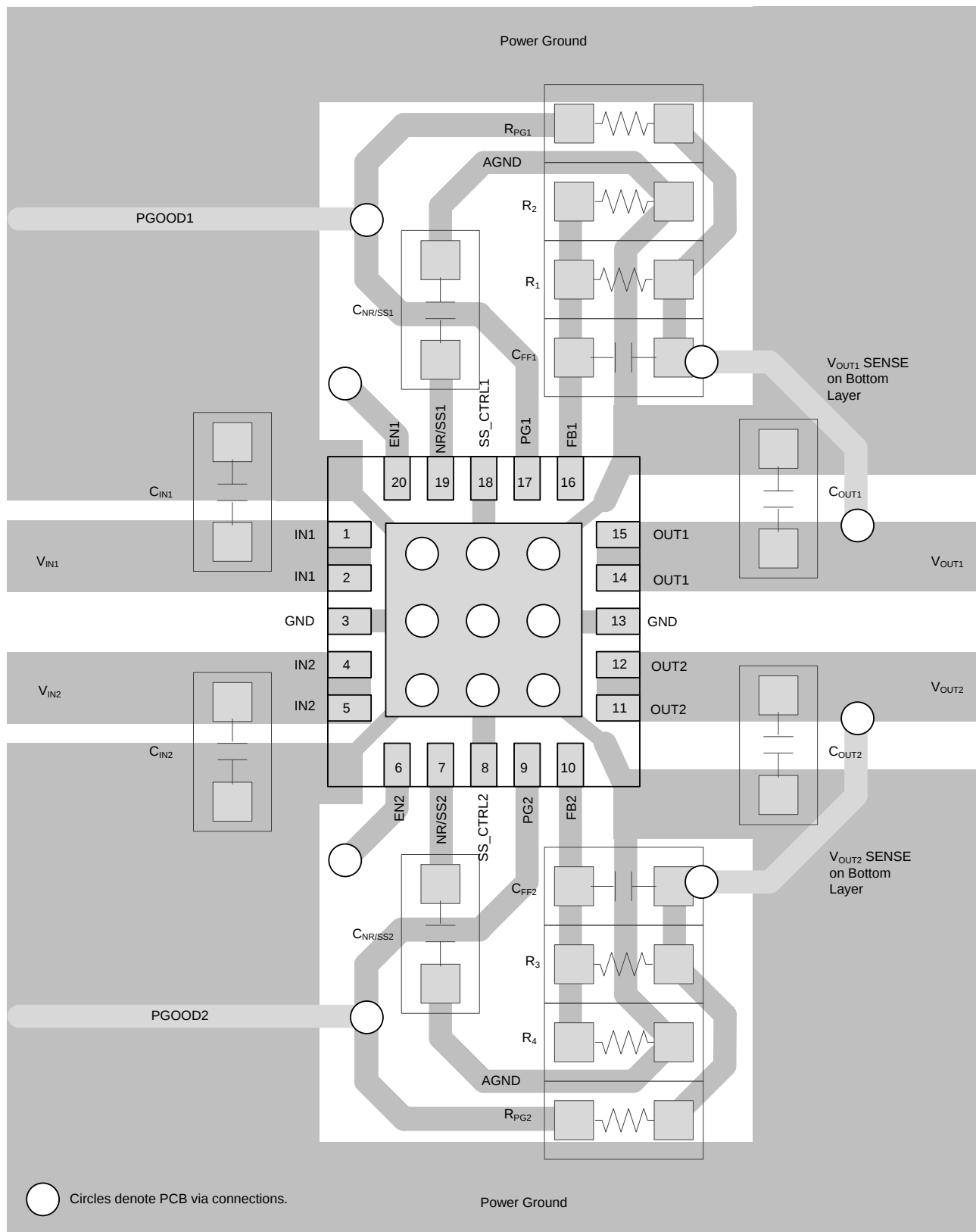
FIG 59. TPS7A88-Q1 Example Layout
