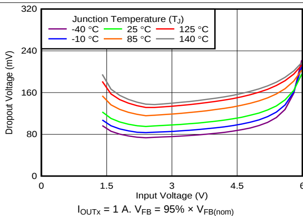
FIG 23. Dropout Voltage vs Input Voltage
