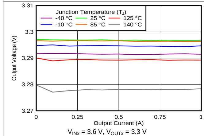
Figure 27. Load Regulation
