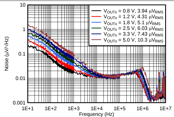
Figure 8. Spectral Noise Density vs Output Voltage
