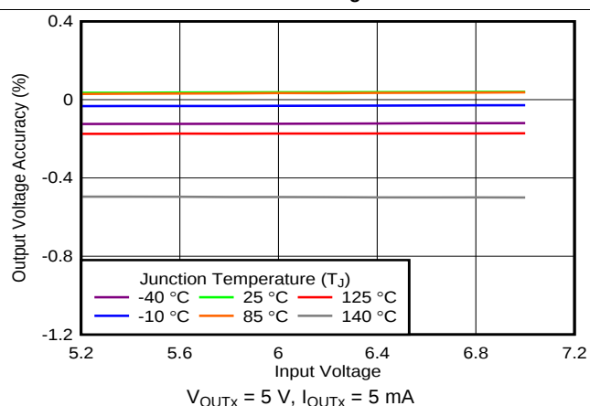
Figure 30. Line Regulation
