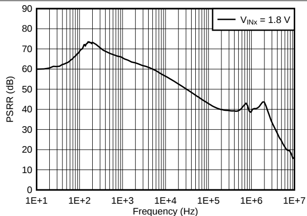
图 56. Power-Supply Rejection
