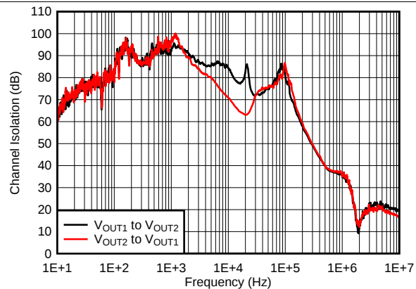
Figure 7. Channel-to-Channel Output Voltage Isolation vs Frequency
