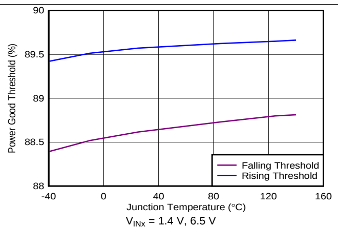
FIG 34. PG Threshold vs Temperature
