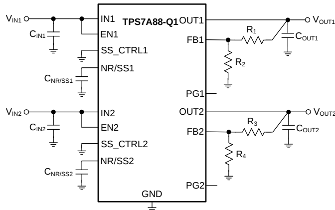
图 45. Adjustable Operation
