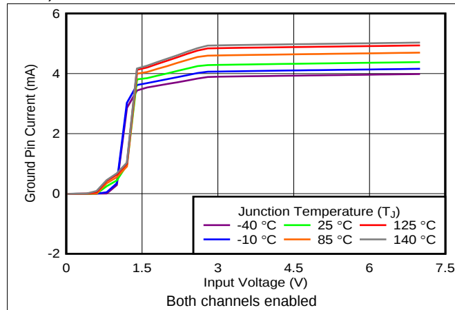
FIG 31. Ground Current vs Input Voltage
