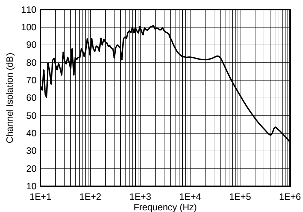
图 57. Channel-to-Channel Isolation
