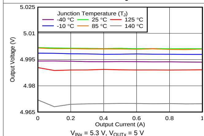
Figure 29. Load Regulation
