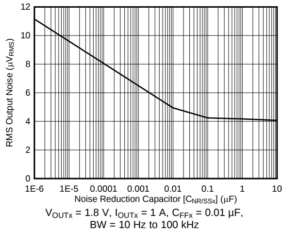
FIG 13. RMS Output Noise vs C_{\text{NR/SSX}}
