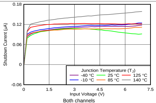
FIG 24. Shutdown Current vs Input Voltage
