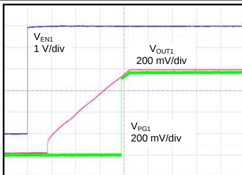
FIG 19. Start-Up
