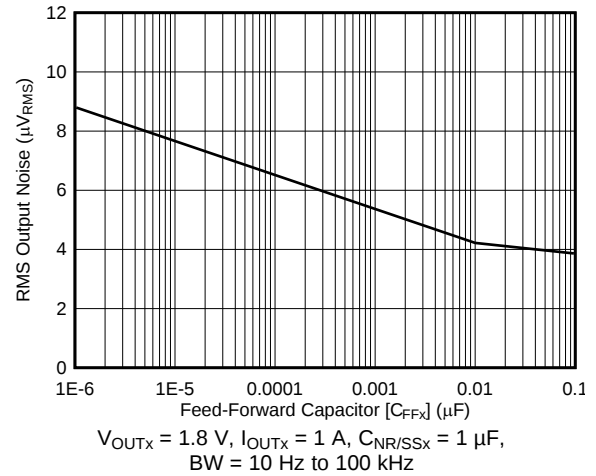
FIG 14. RMS Output Noise vs C_{\text{FFX}}
