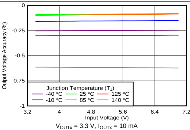
Figure 28. Line Regulation
