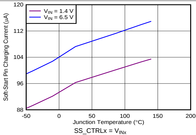
Figure 37. Soft-Start Current vs Temperature
