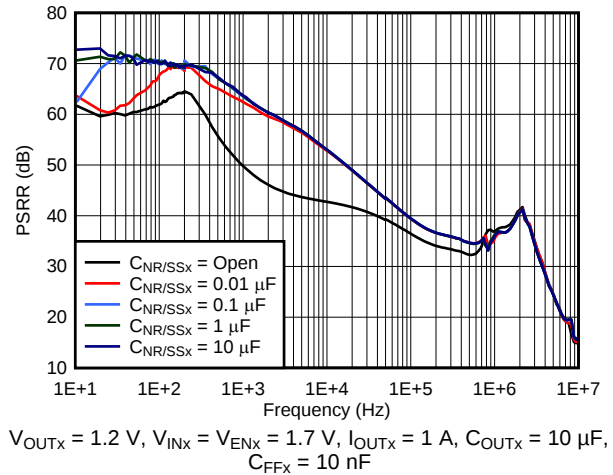
图 2. Power-Supply Rejection vs C_{\text{NR/SSX}}
