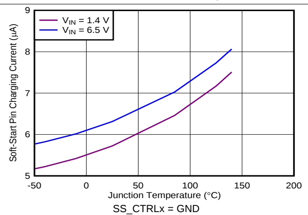
FIG 36. Soft-Start Current vs Temperature
