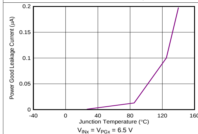
FIG 35. PG Leakage Current vs Temperature
