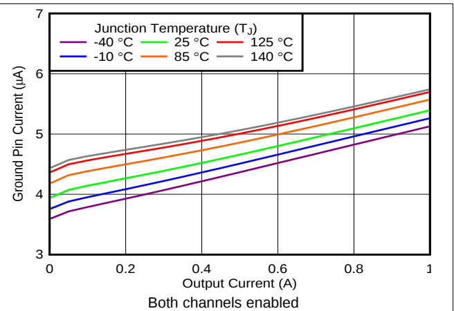
FIG 32. Ground Current vs Output Current
