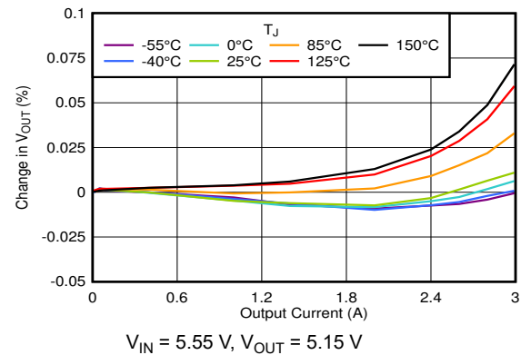
6-74. Load Regulation vs I_{OUT} (5-V Output)
