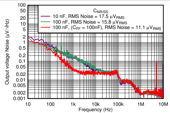
FIG 6-56. Output Noise vs Frequency and C_{NR/SS}
