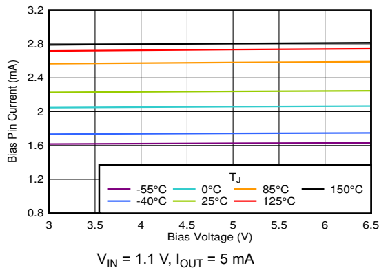
6-79. Bias Pin Current With Bias
