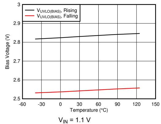
Figure 6-38. V_{BIAS} UVLO vs Temperature
