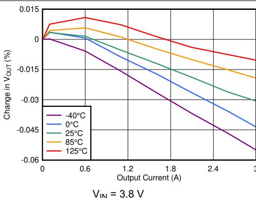
FIG 6-27. Load Regulation vs I_{OUT} (3.3-V Output)
