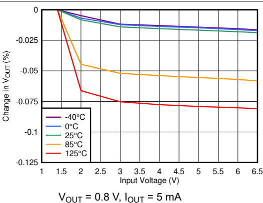
FIG 6-29. Line Regulation vs V_{IN}
