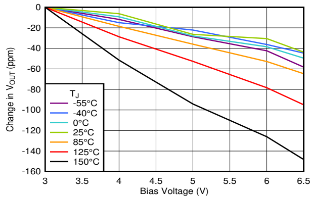
7-55. Line Regulation With BIAS
