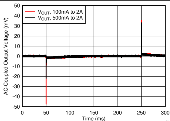
Fig 19. Load Transient vs Time and DC Load
