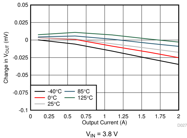
FIG 7-27. Load Regulation (3.3-V Output)
