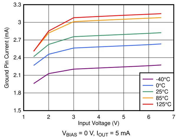
7-32. Ground Pin Current vs Input Voltage
