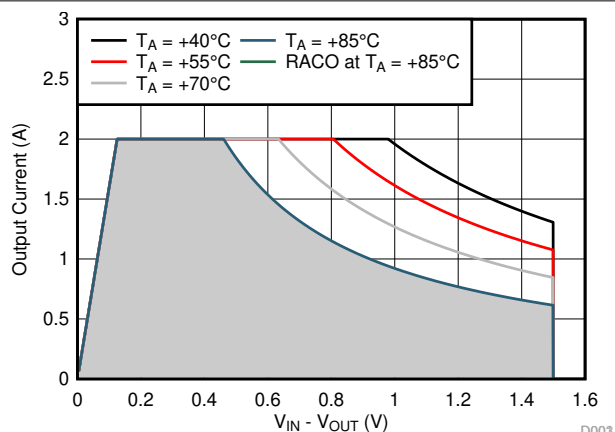
☒ 9-17. Recommended Area for Continuous Operation for V_{OUT} = 1.8\text{ V}
