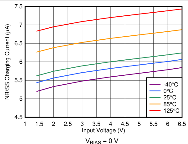
7-36. I_{NR/SS} Current vs Input Voltage
