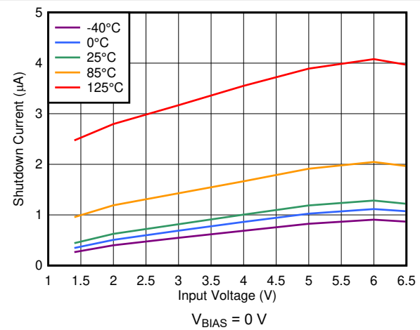
7-34. Shutdown Current vs Input Voltage
