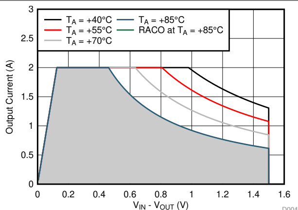
☒ 9-18. Recommended Area for Continuous Operation for V_{OUT} = 2.5\text{ V}
