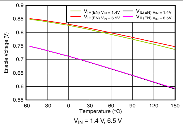
FIG 7-64. Enable Threshold vs Temperature
