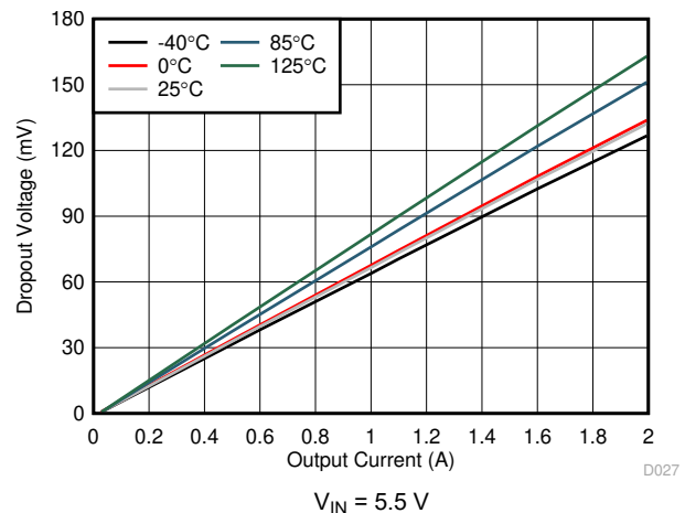
7-50. Dropout Voltage vs Output Current (High V_{IN} )
