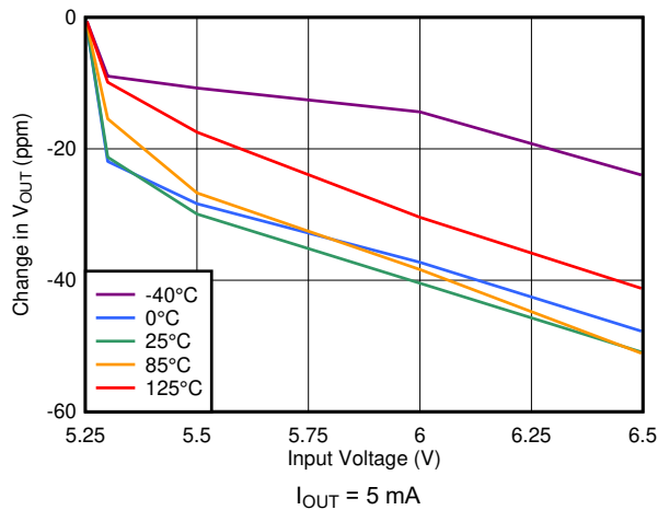
7-31. Line Regulation (5-V Output)
