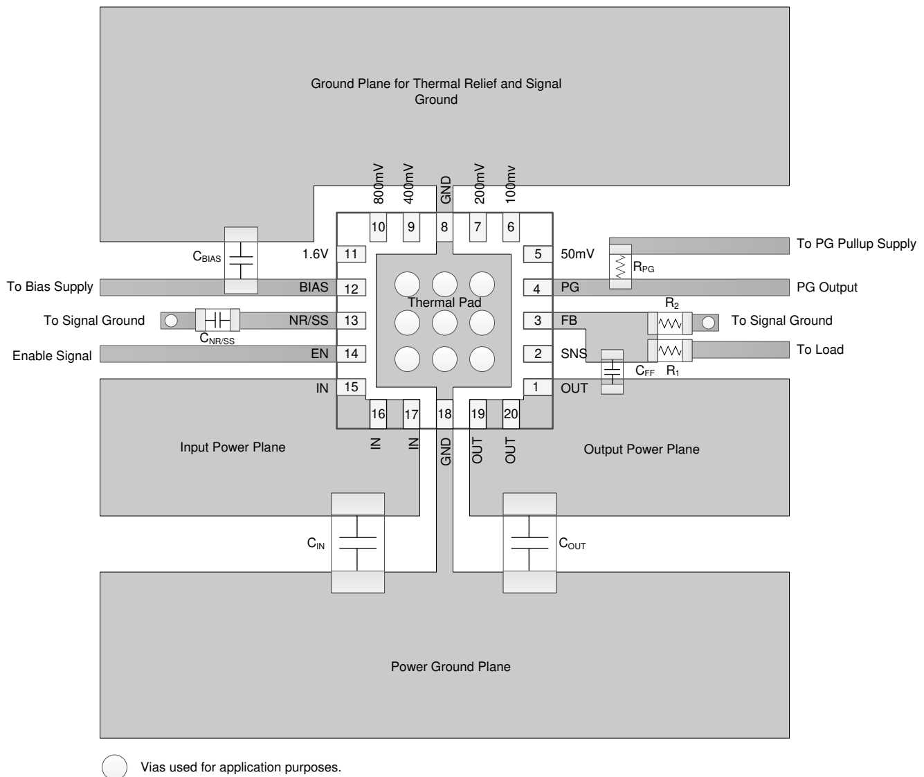
Figure 11-1. Example Layout
