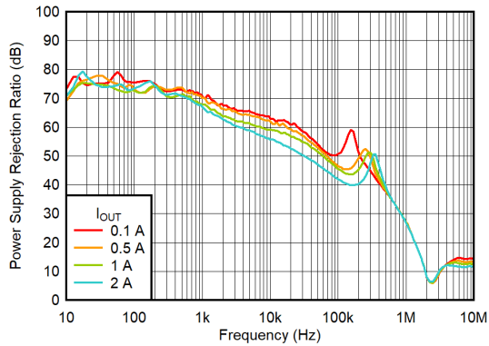
FIG 7-43. PSRR vs Frequency and I_{OUT}
