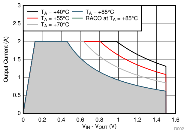
☒ 9-16. Recommended Area for Continuous Operation for V_{OUT} = 1.2\text{ V}
