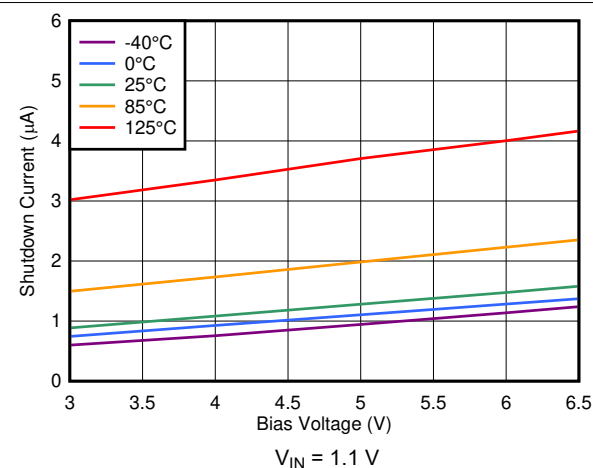
7-35. Shutdown Current vs Bias Voltage
