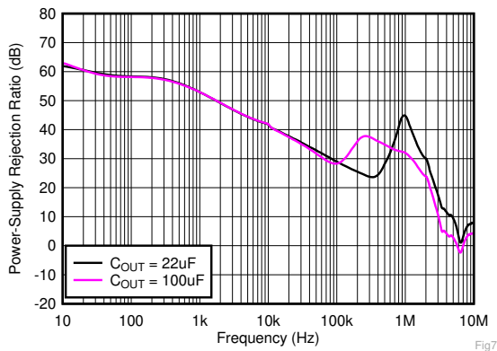
Fig 7-7. PSRR vs Frequency and C_{OUT}
