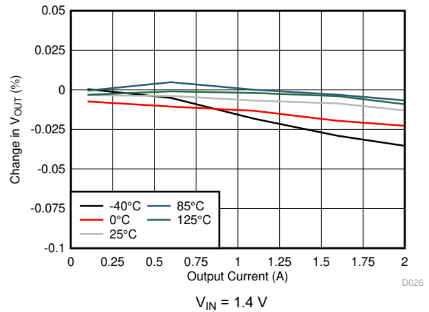
FIG 7-26. Load Regulation
