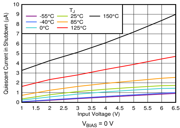
FIG 7-59. Shutdown Current vs Input Voltage
