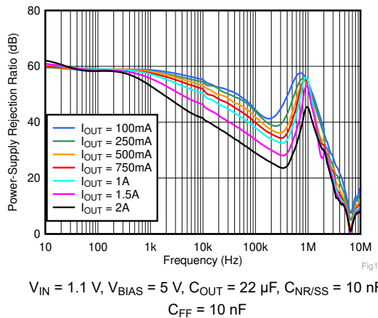
Fig 7-1. PSRR vs Frequency and I_{OUT}
