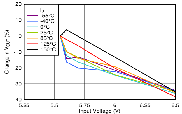
7-54. Line Regulation vs V_{IN}
