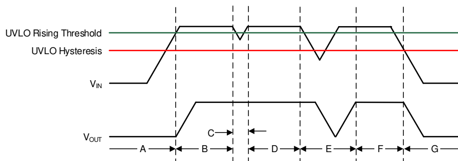
Figure 9-4. Typical UVLO Operation
