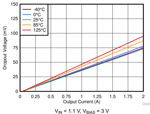
7-49. Dropout Voltage vs Output Current With BIAS
