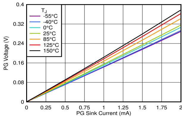
FIG 7-65. PG Voltage vs PG Current Sink
