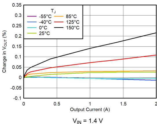
7-51. Load Regulation
