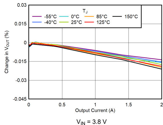
7-52. Load Regulation (3.3-V Output)
