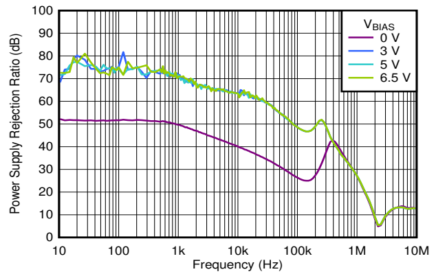
FIG 7-44. PSRR vs Frequency and V_{BIAS}
