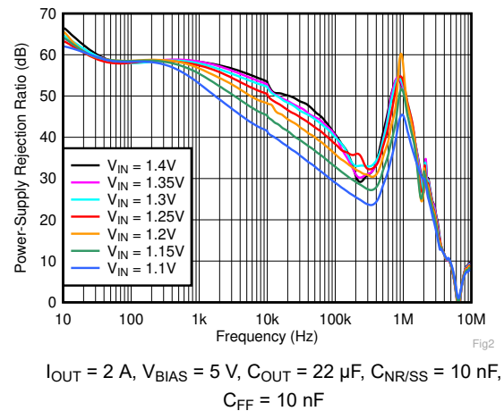
Fig 7-2. PSRR vs Frequency and V_{IN} With BIAS
