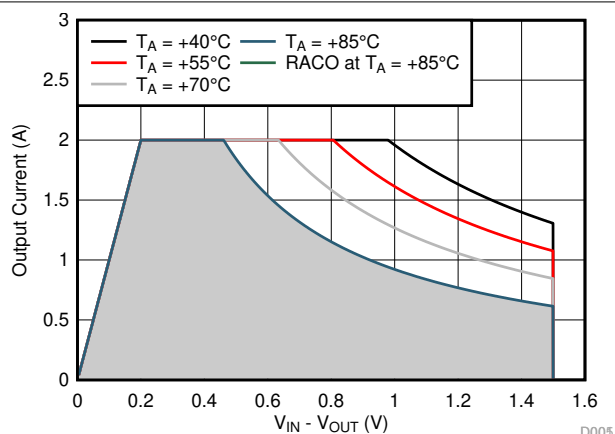
☒ 9-19. Recommended Area for Continuous Operation for V_{OUT} = 3.3\text{ V}
