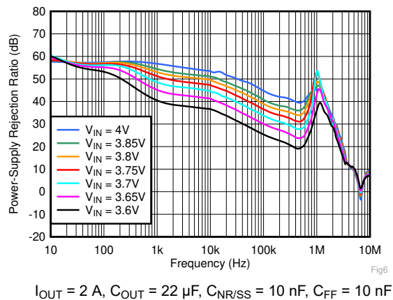
Fig 7-4. PSRR vs Frequency and V_{IN}
