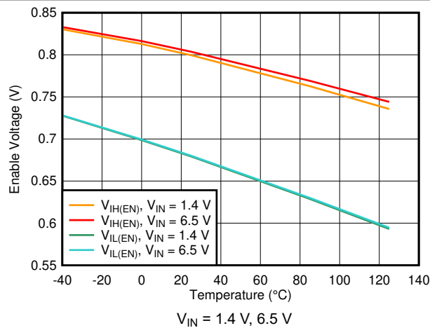
7-39. Enable Threshold vs Temperature
