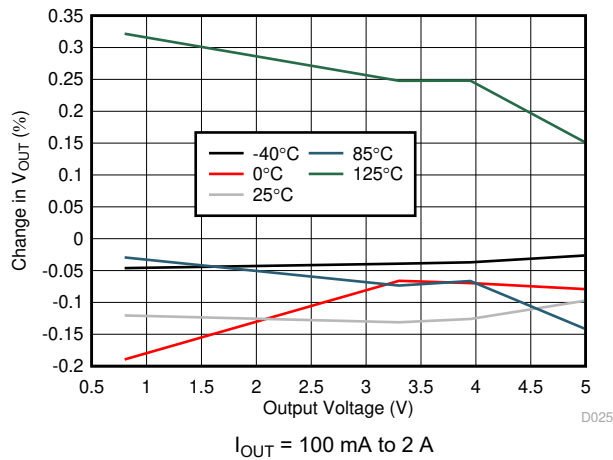
FIG 7-25. Load Regulation vs Output Voltage
