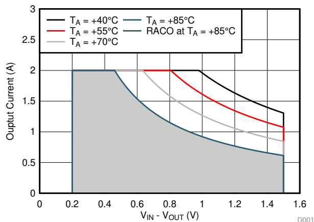
☒ 9-15. Recommended Area for Continuous Operation for V_{OUT} = 0.9\text{ V}
