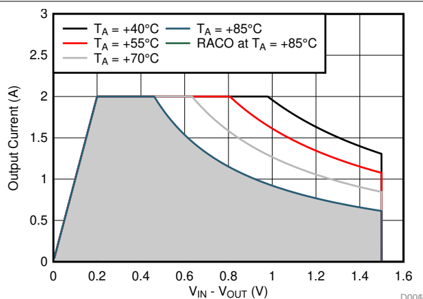
☒ 9-20. Recommended Area for Continuous Operation for V_{OUT} = 5\text{ V}
