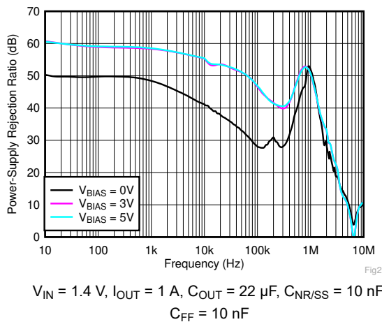
Fig 7-3. PSRR vs Frequency and V_{BIAS}
