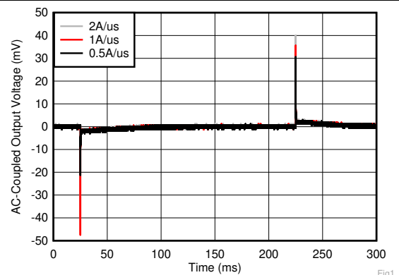
Fig 7-16. Load Transient vs Time for V_{OUT} = 0.8\text{ V}
