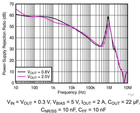
Fig 7-5. PSRR vs Frequency and V_{OUT} With BIAS
