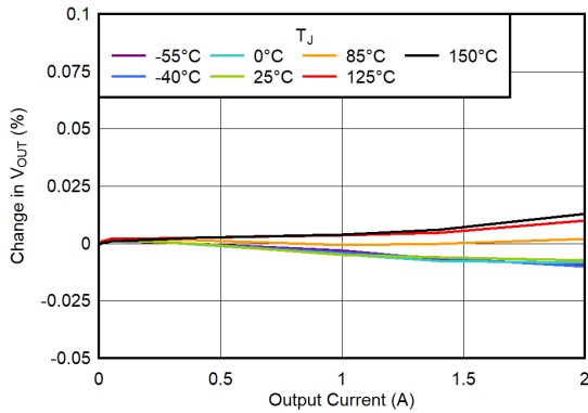
7-53. Load Regulation (5-V Output)
