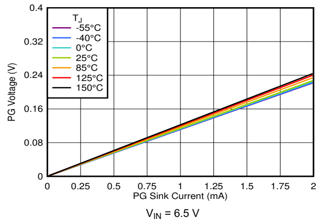
FIG 7-66. PG Voltage vs PG Current Sink
