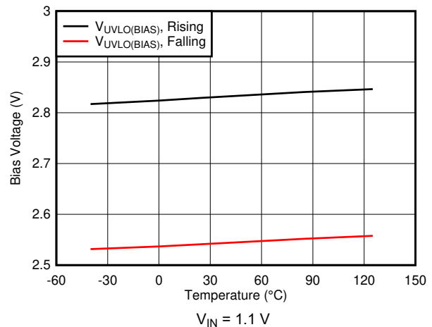
7-38. V_{BIAS} UVLO vs Temperature
