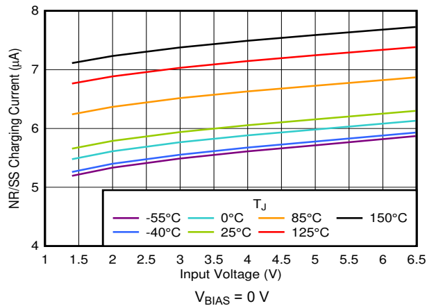
FIG 7-61. I_{NR/SS} Current vs Input Voltage
