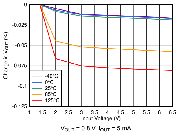
FIG 7-29. Line Regulation
