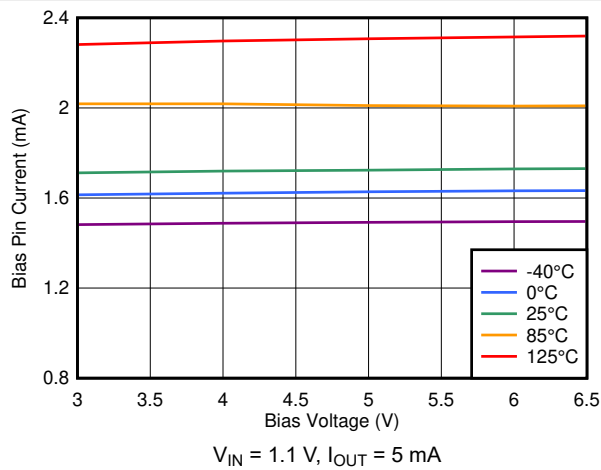
7-33. BIAS Pin Current vs Bias Voltage
