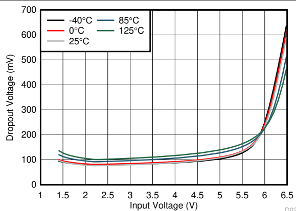
Fig 20. Dropout Voltage vs Input Voltage Without BIAS
