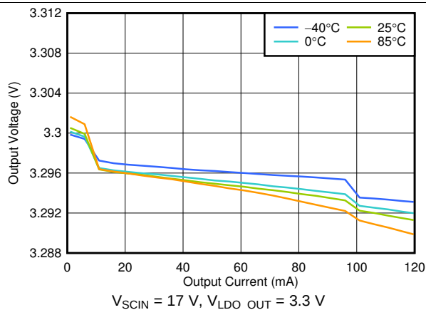
FIG 5. V_{LDO\_OUT} vs I_{OUT} DC Supply on the SCIN Pin
