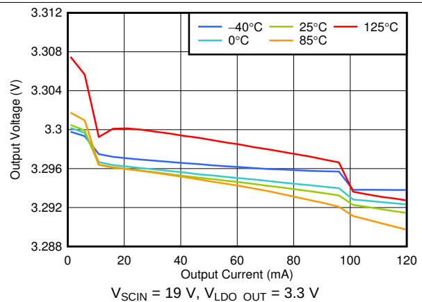
FIG 6. V_{LDO\_OUT} vs I_{OUT} DC Supply on the SCIN Pin
