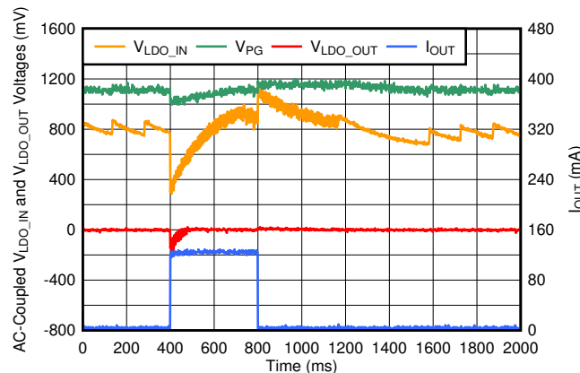
FIG 21. Overvoltage Protection Circuit Behavior for a 5.0-V Output Voltage Device During Load Transient
