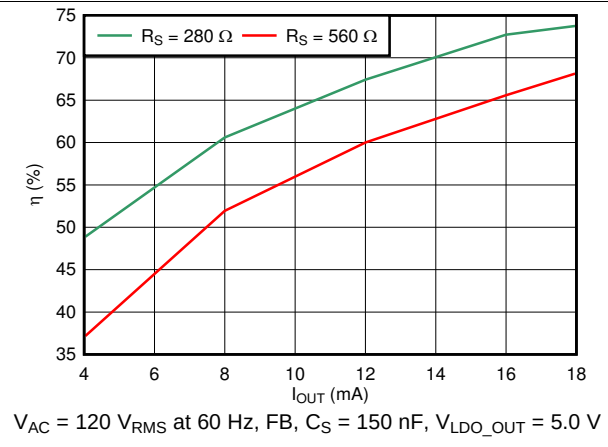
Figure 28. Efficiency vs I_{OUT} FB Configuration
