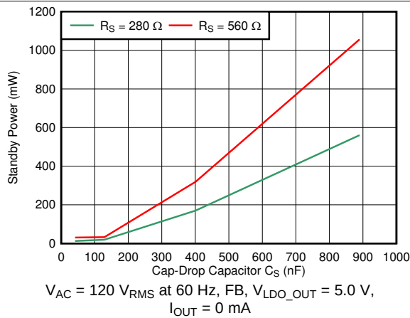
Figure 27. Standby Power vs Cap-Drop Capacitor ( C_S )
