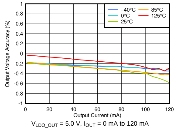
FIG 2. V_{LDO\_OUT} Accuracy vs I_{OUT}
