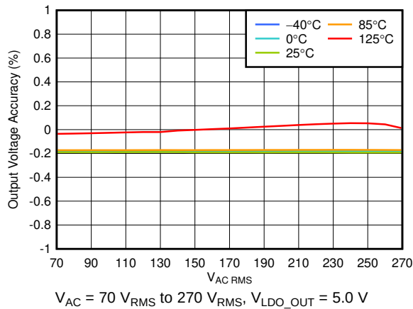
FIG 1. V_{LDO\_OUT} Accuracy vs V_{AC} Supply
