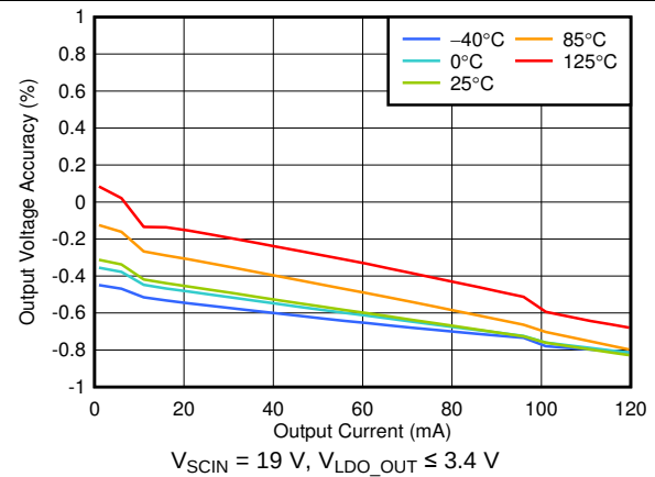
FIG 4. V_{LDO\_OUT} Accuracy vs I_{OUT} DC Supply on the SCIN Pin
