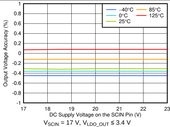
FIG 3. V_{LDO\_OUT} Accuracy vs DC Supply on the SCIN Pin
