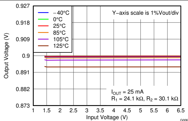
5-7. Line Regulation (0.9 V, Adjustable)
