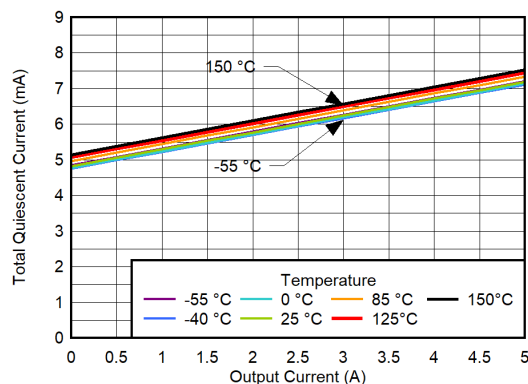
FIG 6-144. Total Quiescent Current vs I_{OUT} for V_{OUT} = 5.2\text{ V} , V_{BIAS} = 11\text{ V} , CP Disabled
