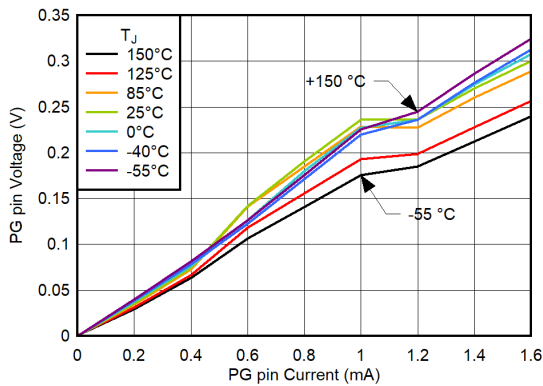
FIG 6-225. PG Pin Low-Level Voltage vs PG Pin Current for V_{IN} = 0.7 V, V_{BIAS} = 3 V, V_{CP\_EN} = 1.8 V
