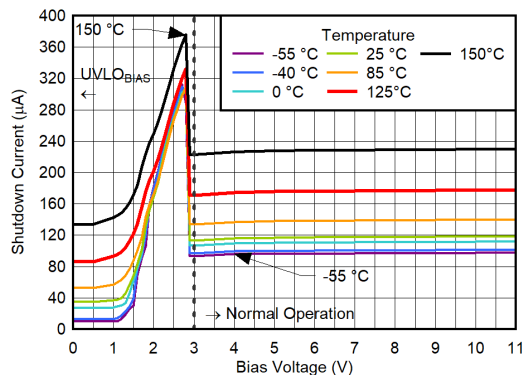
FIG 6-202. BIAS Pin Shutdown Current vs V_{BIAS} for V_{IN} = 0.7 V, V_{OUT(nom)} = 0.5 V, CP Disabled
