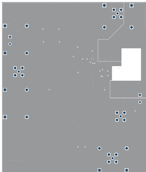
✎ 8-31. Layer 2 Routing
