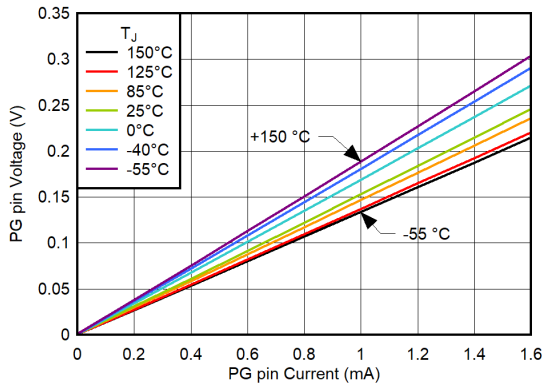
FIG 6-223. PG Pin Low-Level Voltage vs PG Pin Current for V_{IN} = 0.7 V, V_{BIAS} = 3.7 V, V_{CP\_EN} = 0 V
