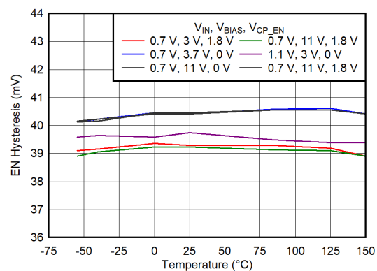
FIG 6-210. EN Hysteresis vs Temperature for V_{IN} = 0.7\text{ V} and 1.1\text{ V} , V_{OUT} = 0.5\text{ V}
