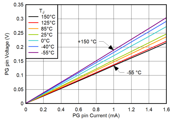
FIG 6-226. PG Pin Low-Level Voltage vs PG Pin Current for V_{IN} = 0.7 V, V_{BIAS} = 11 V, V_{CP\_EN} = 1.8 V
