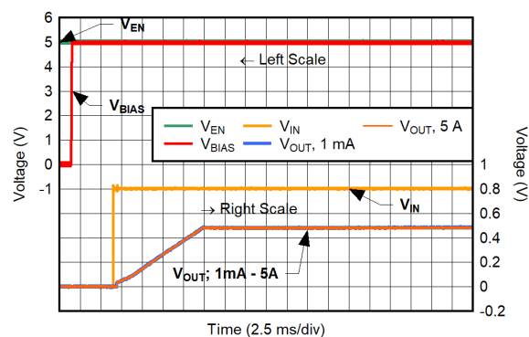
6-52. Start-Up Under Current Limit
