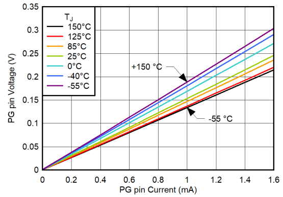
FIG 6-224. PG Pin Low-Level Voltage vs PG Pin Current for V_{IN} = 0.7 V, V_{BIAS} = 11 V, V_{CP\_EN} = 0 V
