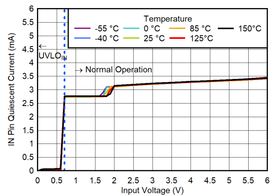
FIG 6-148. IN Pin Quiescent Current vs V_{IN} for V_{OUT} = 0.5\text{ V} , V_{BIAS} = 11\text{ V} , CP Disabled
