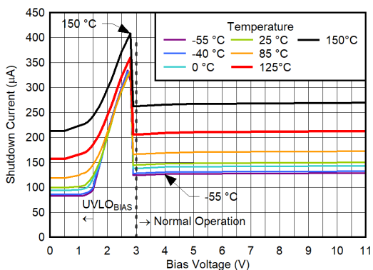
FIG 6-201. Total Shutdown Current vs V_{BIAS} for V_{IN} = 6 V, V_{OUT(nom)} = 0.5 V, CP Enabled
