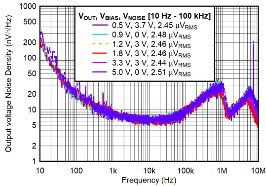
Figure 6-29. Output Voltage Noise Density vs Frequency and V_{OUT} for CP Enabled
