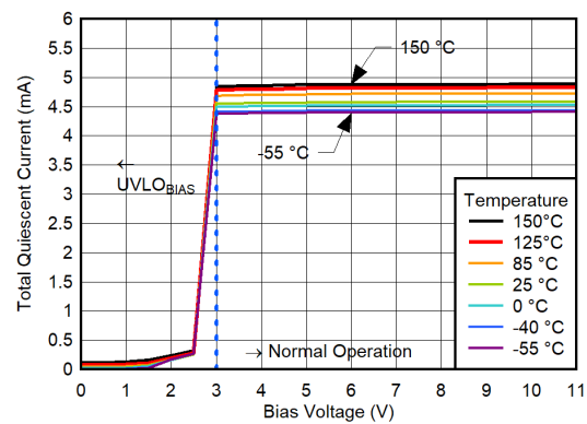
FIG 6-178. Total Quiescent Current vs V_{BIAS} for V_{OUT} = 0.5 \text{ V} , V_{IN} = 0.7 \text{ V} , CP Disabled, I_{OUT} = 0 \text{ A}
