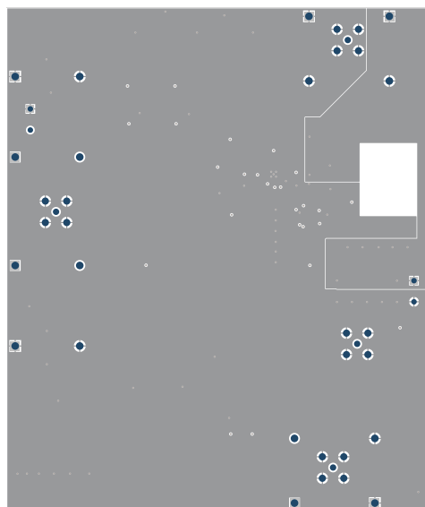
✎ 8-34. Layer 5 Routing
