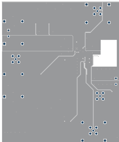
✎ 8-32. Layer 3 Routing
