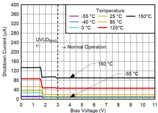
FIG 6-201. Total Shutdown Current vs V_{BIAS} for V_{IN} = 6 V, V_{OUT(nom)} = 0.5 V, CP Enabled
