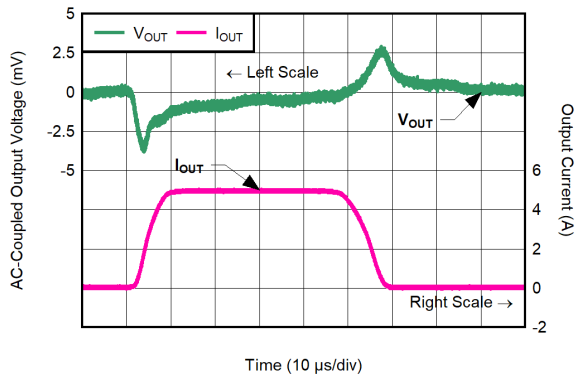
6-45. Load Transient for V_{OUT} = 5.2\text{ V} , I_{OUT} = 100\text{ mA} to 5\text{ A} , CP Disabled, SR = 5\text{ A}/\mu\text{s} , V_{BIAS} = 8.4\text{ V}
