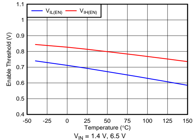
34. Enable Threshold vs Temperature
