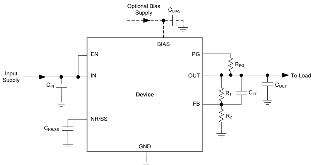
Figure 43. Adjustable Operation
