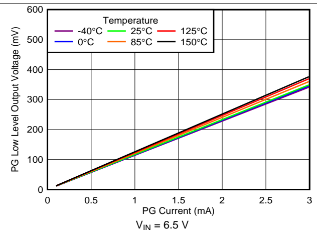
36. PG Voltage vs PG Current Sink
