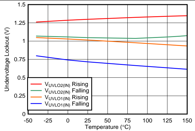
32. V_{IN} UVLO vs Temperature
