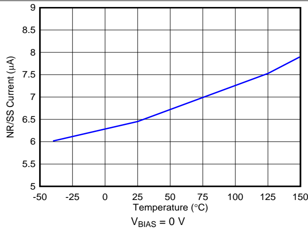
31. NR/SS Current vs Temperature
